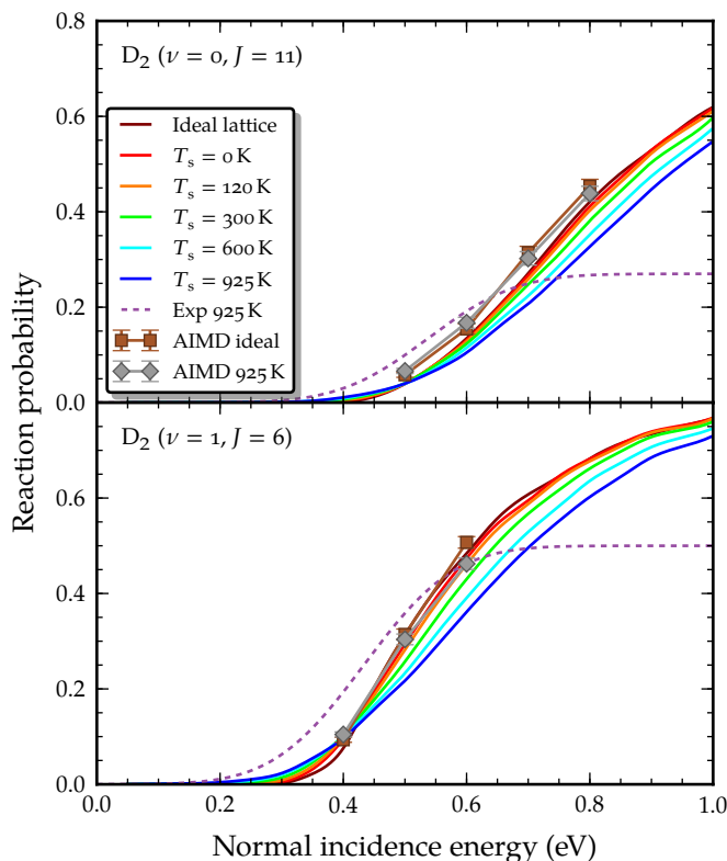
FIGURE 3.4 Broadening of the sticking curve for D_2 initially in the (\nu = 0, J = 11) and (\nu = 1, J = 6) states, for all considered surface temperatures, only taking into account the effects of thermal displacement. The experimental sticking curve 29 is also plotted, as well as the AIMD results by NATTINO et al. 20
