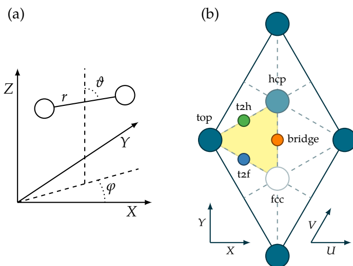
FIGURE 5.2 (a) Coordinate system for dissociation of H 2 on a surface. In the plot, X, Y, and Z are the center of mass coordinates of H 2 , r is the H–H distance, \theta is the polar angle of the molecular axis with the Z-axis, and \varphi is the azimuthal angle. (b) Schematic representation of the unit cell with the high symmetry sites on the Pd(111) surface, and of considered H 2 –surface geometries.
