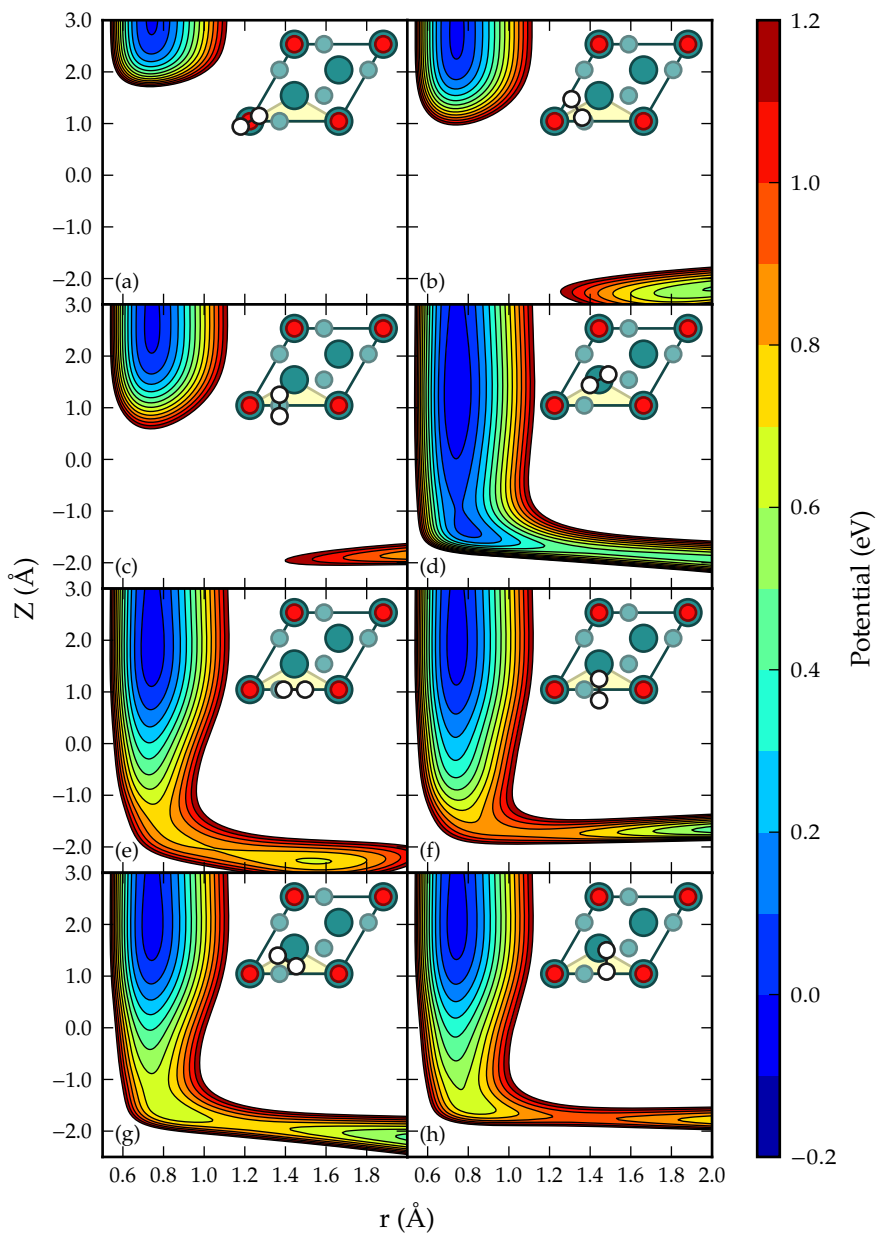
FIGURE 7.4 The (r, Z) dependence of the PES for H_2 dissociating on 1/3 ML CO-covered Ru(0001) above several different sites and orientations ( \vartheta = 90^\circ ). (a) top_{ads} ( \varphi = 0^\circ ), (b) bridge_{ads} ( \varphi = 120^\circ ), (c) hcp ( \varphi = 90^\circ ), (d) top ( \varphi = 0^\circ ), (e) bridge ( \varphi = 0^\circ ), (f) bridge ( \varphi = 90^\circ ), (g) t2h ( \varphi = 150^\circ ), (h) t2f ( \varphi = 90^\circ ).
