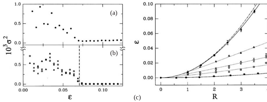
Fig. 39. Various data from the experiments of Babcock et al. [19]. (a) (Upper left panel) Normalized mean squared width \sigma^2 of the peak in the frequency spectrum as a function of \epsilon at Re = 3 obtained from the measurement of the pattern amplitude as a function of time at a position 100d behind the inlet (note that this is three times further from the inlet than the region shown in Fig. 38(a)). The sharp transition at \epsilon = 0.065 indicates the change from the small- \epsilon regime where the patterns are incoherent due to phase noise to a coherent large- \epsilon regime where pattern are coherent. This value is therefore associated with the transition from the convectively unstable to the absolutely unstable regime. (b) (Lower left panel) Corresponding results for the CGL equation (137) with three different noise levels, 10^{-6} ( \times ), 10^{-5} ( \triangle ), and 10^{-4} ( \circ ). The dashed line locates the transition \epsilon_{ca}^{CGL} = 0.071 [19]. (c) Stability diagram for axisymmetric Taylor vortex patterns. The lower line and data points mark the line \epsilon_c(Re) where the instability sets in. The upper data points locate the transition \epsilon_{ca} from the convectively unstable regime to the absolutely unstable regime as determined from the change-over from coherent to incoherent patterns via measurements of the spectrum like those in (a), while the dashed line indicates \epsilon_{ca}^{CGL} . Between the lower line and the upper line, the system is convectively unstable, and noise-sustained structures like those in the one but lowest panel of Fig. 38 occur. Open symbols indicate the boundaries where noise sustained structures occur in simulations, from top to bottom, at z = 25d , 50d , and 100d . The dotted lines indicate estimates of these boundaries from the deterministic CGL equation (137) with a fixed value of A(z = 0) imposed.
