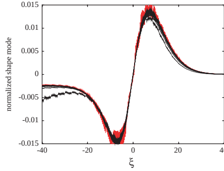
Fig. 57. Demonstration of the universal relaxation behavior of the shape of a front in the Swift–Hohenberg equation (92), according to Spruijt et al. [147,383]. Plotted is ratio (215) for times 20–160 in steps of 20 for fronts in numerical simulations of fronts in for \varepsilon = 1/2 . The fact that the various curves fall almost on top of each other confirms that the shape of the fronts follows the relaxation of the velocity adiabatically. The curve which deviates somewhat on the left side is taken at the earliest time, t = 20 . Up to an overall multiplicative constant, the resulting curve represents the shape mode of the pulled Swift–Hohenberg front. Note that since \varepsilon is not small, various harmonics contribute to the expansion of the asymptotic profile, and the front solution is not close to the front solution of the cubic amplitude equation that one can derive in the limit 0 < \varepsilon \ll 1 .
