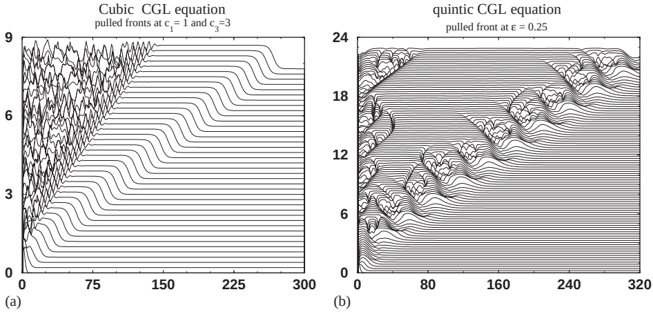
Fig. 17. (a) Space–time plot of the amplitude A in a simulation of the cubic GL equation (97) with \varepsilon=1 , c_1=1 and c_3=3 . Time difference between successive lines is 2 and the total simulation time is 80. The plot illustrates how the first front is a pulled coherent pattern forming front of the type (101), but that the state behind the front is unstable, so that the domain with the state selected by the first front is invaded by a second front. This second front is also a pulled one. Note the similarity between the leading part of the second front and the pulled front found in the Kuramoto–Sivashinsky equation—see Fig. 16(a). This is no accident, as the Kuramoto–Sivashinsky equation is the lowest order amplitude equation just above the Benjamin–Feir instability [105,189]. (b) Space–time plot of a propagating pulled front in the quintic CGL equation with \varepsilon=0.25 , c_1=1 , c_3=-1 and c_5=-1 . For these parameter values, no coherent nonlinear front solution of the type (101) exists [424]. The first front is followed by a region with phase slips (points where A vanishes), before giving rise to a state close to a phase-winding solution. At the later stage, this region is invaded by another front.
