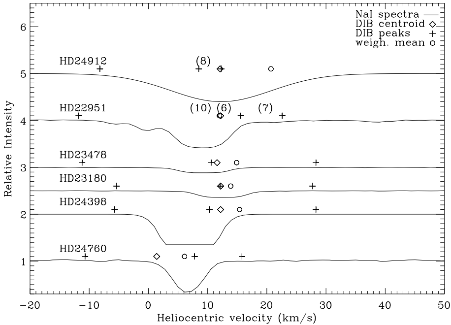
Fig. 7. High resolution Na I spectra (except for HD24912 R=25000 ) obtained during our campaigns. HD24398 was taken from Welty et al. (1994). Velocities are heliocentric.
