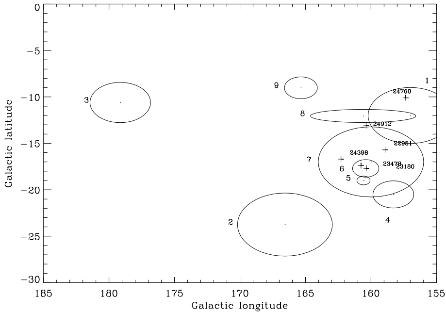
Fig. 2. Sketch of the cloud distribution in Perseus OB2 in galactic coordinates. The program star location is indicated with a (+). The cloud numbering is: (1) dark clouds around TMC-1, (2) Merope nebulae, (3) dark clouds around NGC1750/58, (4) NGC1333, (5) Barnard dark cloud B1, (6) IC348 dark cloud, (7) Per OB2 H I shell, (8) NGC1499, (9) NGC1579, (10) cloud stripe extending from HD23180 to HD24912 seen on IRAS 60 \mu maps, not reported for clarity.
