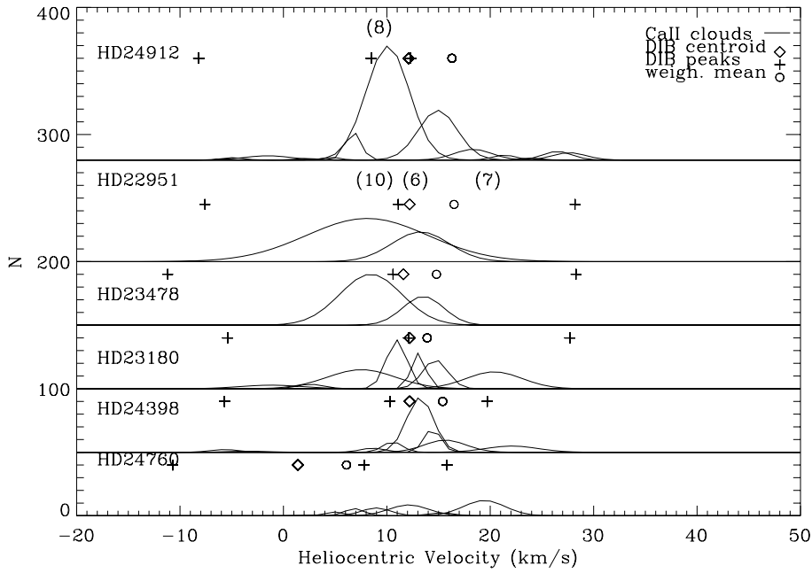
Fig. 6. The Ca II multiple cloud column density distribution ( N ) along the program star lines of sight. The diamond indicates the position of the DIB cloud using ( V_C ). The empty circle is the DIB weighted mean velocity V_{\text{DIBwm}} . We also reported the positions of clouds (6), (7), (8) and (10) showing the spatial link with some Ca II components.
