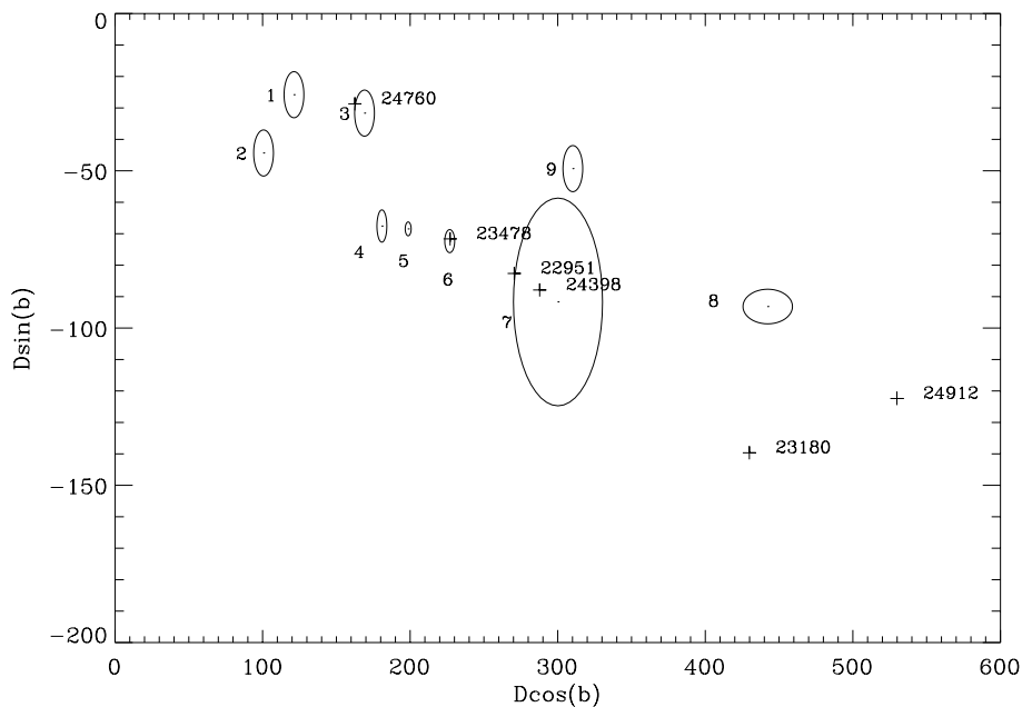
Fig. 3. Sketch of the clouds distribution in Perseus OB2 in a galactic cartesian diagram. The program star location is indicated with a (+). The cloud numbering is identical to Fig. 2.
