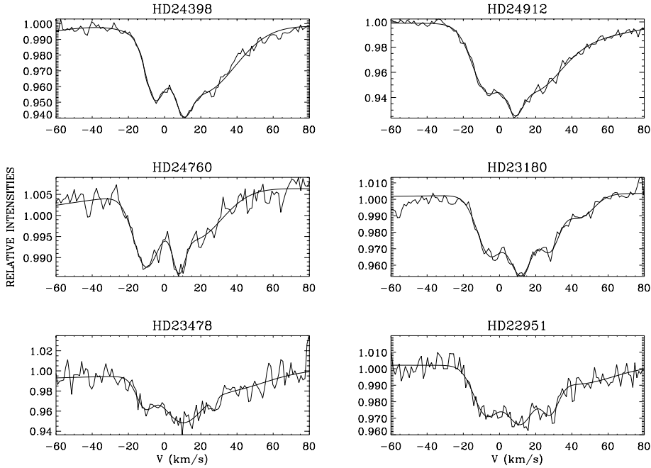
Fig. 1. The \lambda 6613 \text{ \AA} DIB profiles toward the observed Perseus lines of sight together with their corresponding fits. The velocities are heliocentric and can be compared with the Ca II velocities (Fig. 6). This confirms that the triple peak substructures are intrinsic to the DIB (rotational contour of gas phase molecule) and not due to multiple cloud Doppler effects. Stars are named according to their HD numbers.
