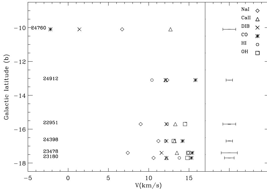
Fig. 5. The \lambda 6613 \text{ \AA} DIB centroid distribution together with the Ca II, Na I, H I, OH and CO distributions vs star galactic latitude. The velocities are heliocentric. The DIB ( 1\sigma ) error measurements are reported on the right part of the diagram together with the interstellar species symbols. The targets HD number are reported on the left side. HD22951 was displaced in +1 degree in galactic latitude for clarity.
