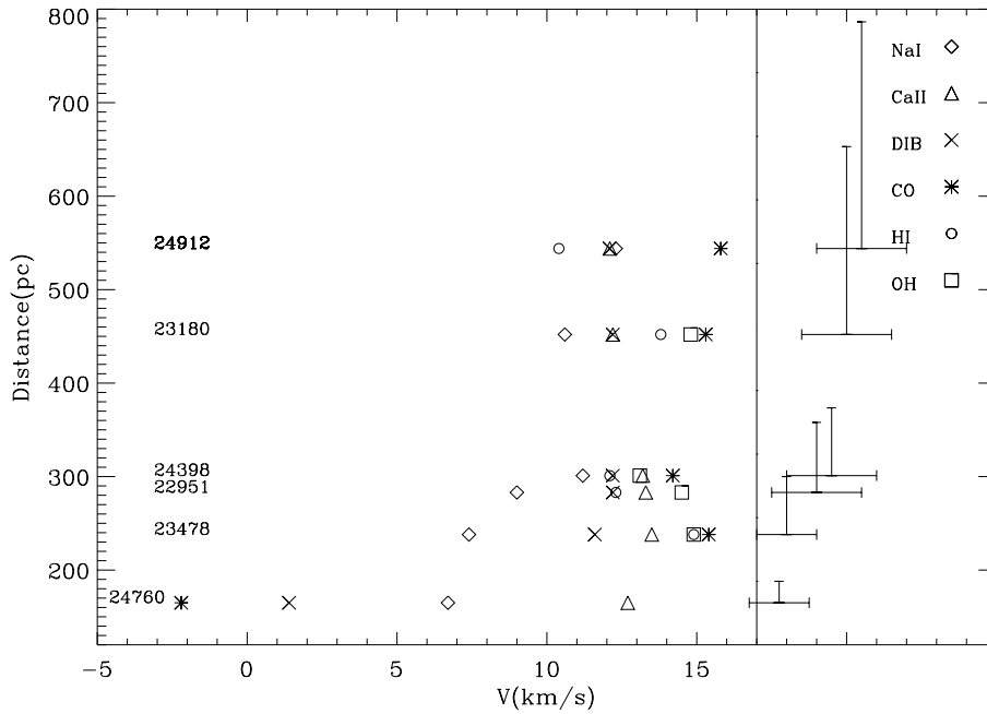
Fig. 4. The \lambda 6613 \text{ \AA} DIB centroid distribution together with the Ca II, Na I, H I, OH and CO distributions vs star Hipparcos distance. The DIB and distance error measurements are reported on the right part of the diagram together with the interstellar species symbols. Velocities are heliocentric. The targets HD number are reported on the left side.
