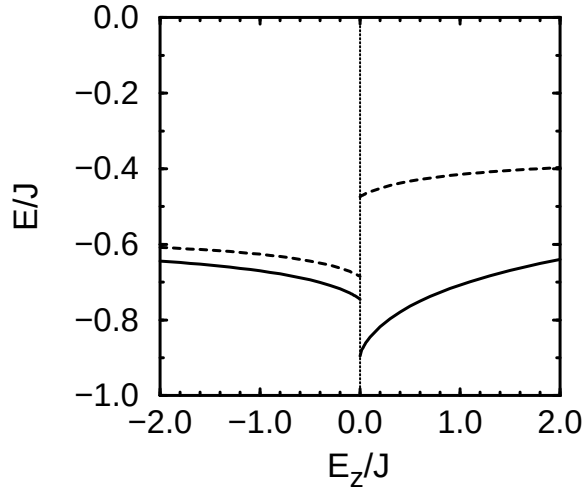
Figure 4. Ground state energies E of the AF zz (left) and AF xx (right) phases as functions of E_z/J , obtained using the RPA (full lines) and the SW+SWO scheme (dashed lines).
