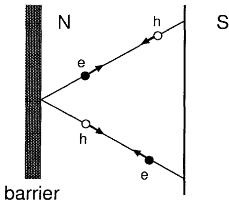
Figure 4.5 Periodic orbit consisting of two normal reflections and two retro-reflections. The net phase increment is zero in the optical case and -\pi in the electronic case. Hence the periodic orbits interfere constructively for light and destructively for electrons. This explains why the barrier becomes transparent for light but not for electrons.
