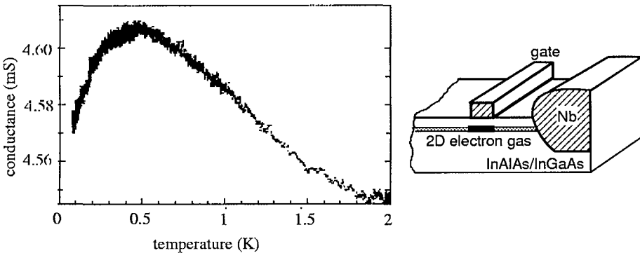
Figure 4.4 Temperature dependence of the conductance of an NS junction, showing the re-entrance effect. The superconductor is Nb, the normal metal is a two-dimensional electron gas. A gate creates a strongly disordered region in the 2D gas that dominates the conductance of the junction. Upon lowering the temperature the conductance first rises and then drops again. Under ideal circumstances the low- and high-temperature limits would be the same. From Ref. [16].
