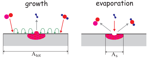
Fig. 1. Sketch of the surface chemical processes involved in the growth and evaporation of an island of solid material s at the surface of a dirty dust grain. The total surface area A_{\text{tot}} of the grain collects molecules which are then transported by hopping to meet on the island’s surface area A_s , where the actual chemisorption process can take place.
