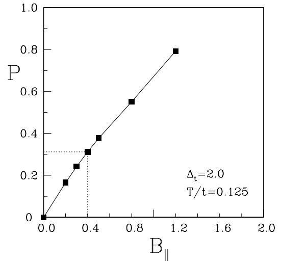
FIG. 4. Degree of spin polarization P = (n_{\uparrow} - n_{\downarrow})/(n_{\uparrow} + n_{\downarrow}) (see text) as a function of B_{||} for fixed low T = t/8 . The polarization shows little change through the metal-insulator transition and is only 0.31 at the estimated critical field strength.
