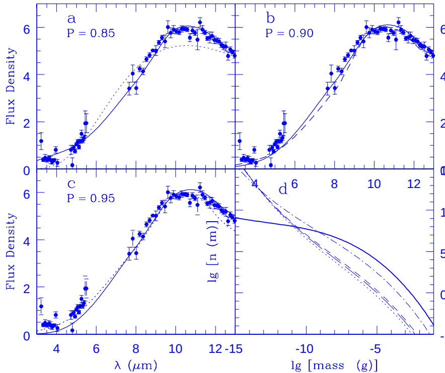
Fig. 2a–d. The theoretical spectra calculated for the porous aggregate comet dust model of silicate core- amorphous carbon mantle grains with a porosity P = 0.85 (a, \chi^2 \simeq 4.5 ), 0.90 (solid line in b, \chi^2 \simeq 6.6 ), and 0.95 (c). The dotted line in a is a black-body ( T = 275 K) emission (Hanner et al. 1996). Also plotted in b (dashed line, \chi^2 \simeq 10.5 ) is the spectrum produced by the P = 0.90 model with a thinner mantle ( m_{\text{or}}/m_{\text{si}} = 1/2 ) and with the same size distribution as for the P = 0.85 model (dotted line in d). In c, both the solid line ( \chi^2 \simeq 7.8 ) and the dotted line ( \chi^2 \simeq 9.1 ) are model spectra for P = 0.95 . The corresponding dust size distributions are shown in d: solid – the Halley dust size distribution; dotted – P = 0.85 ; short dashed – P = 0.90 ; long dashed – P = 0.95 (corresponding to the dotted curve in c); dotted – short dashed – P = 0.95 (corresponding to the solid curve in c).
