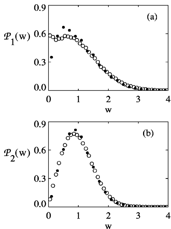
FIG. 6. Direct comparison of (a) \mathcal{P}_1(w) and (b) \mathcal{P}_2(w) for bulk (open circles) and bottom particles (dots). All distributions are scaled such that \langle w \rangle = 1 .
