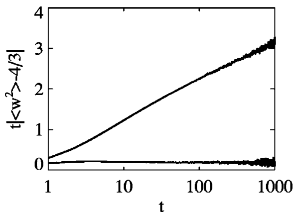
FIG. 12. Relaxation of the second moments with injection (climbing line) and without injection (flat line) towards their asymptotic values 4/3 in the 3D q model. Since we plot t|\langle w^2 \rangle^{(t)} - 4/3| along the vertical axis, the climbing straight line confirms the \log(t)/t relaxation for the q model with injection. Without injection the relaxation is simply 1/t .
