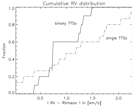
Fig. 3. Cumulative RV distributions for T Tauri “singles” (dash-dotted line) and binaries/multiples (solid line). Note the steeper rise of the binary subsample indicating an absence of a high velocity tail compared to those T Tauri stars regarded as single.
