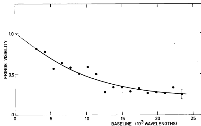
Fig. 8. Fringe visibility curve of NGC 2146 in position angle 36^{\circ} (averaged over 5^{\circ} in position angle). The \pm 1\sigma error bars are shown on the longest baseline data point. The extrapolation to zero spacing is based on short baseline data in that part of the U-V plane where instrumental effects are unimportant
