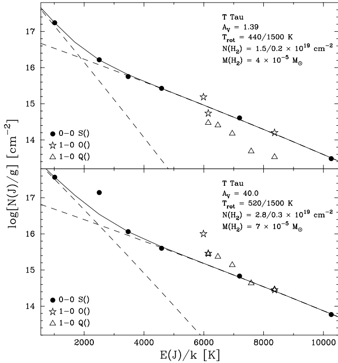
Fig. 5. H 2 excitation diagrams for T Tau, with the data corrected for extinction with A_V = 1^m39 (top) and A_V = 40^m0 (bottom). For most measurements, formal errors are about the size of the plot symbol. The dashed lines give the Boltzmann distribution fits to the two components of thermal H 2 emission. The solid line shows the sum of both components.
