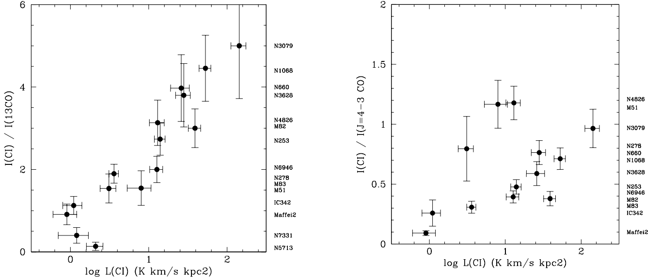
Fig. 2. Left: [\text{CI}]/(J = 2-1^{13}\text{CO}) ratios versus area-integrated [\text{CI}] luminosity L[\text{CI}] . Right: [\text{CI}]/(J = 4-3^{12}\text{CO}) ratios versus L[\text{CI}] . The I([\text{CI}])/I(^{13}\text{CO}) ratio appears to be a well-defined function of \log L([\text{CI}]) ; the I([\text{CI}])/I(4-3^{12}\text{CO}) ratio is not. Galactic sources (not shown) would all be crowded together in the lower left corner.
