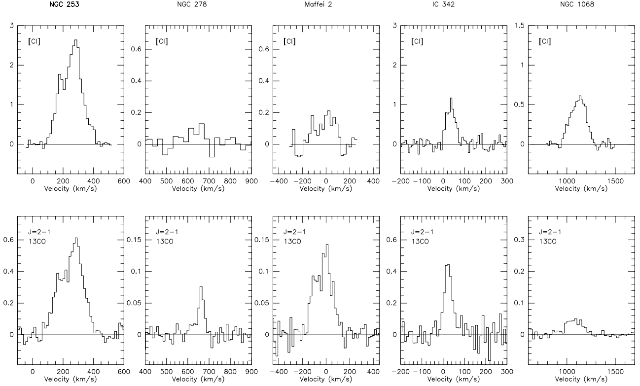
Fig. 1. [C I] and J = 2-1 ^{13}\text{CO} spectra observed towards sample galaxies. The vertical scale is T_{\text{mb}} in K; the horizontal scale is velocity V_{\text{LSR}} in \text{km s}^{-1} . For all galaxies, the temperature range in [C I] is four times that in ^{13}\text{CO} .
