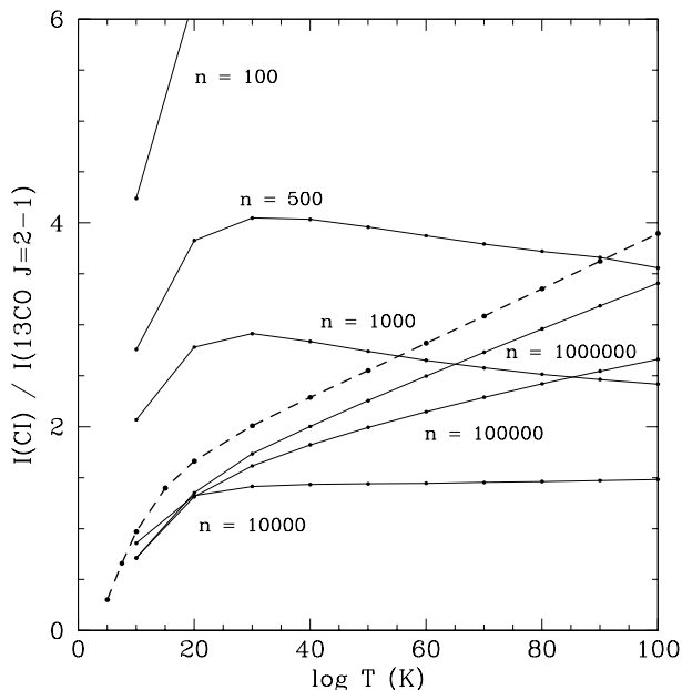
Fig. 3. Model line ratio I(\text{CI})/I(J=2-1^{13}\text{CO}) versus T_{\text{kin}} resulting for equal column densities N(\text{CI})/dV = N(\text{CO})/dV (solid lines). Curves for a range of total gas densities are marked in particles per cc. Dashed line: the ratio I(\text{CI})/I(J=2-1^{13}\text{CO}) versus T_{\text{ex}} , likewise requiring equal column densities N(\text{CI})/dV = N(\text{CO})/dV but assuming optically thin LTE conditions.
