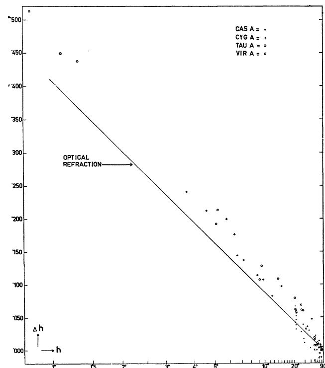
Deviation \Delta h from the standard position of radio stars. The scale of abscissae is chosen so as to make the optical refraction curve a straight line.
