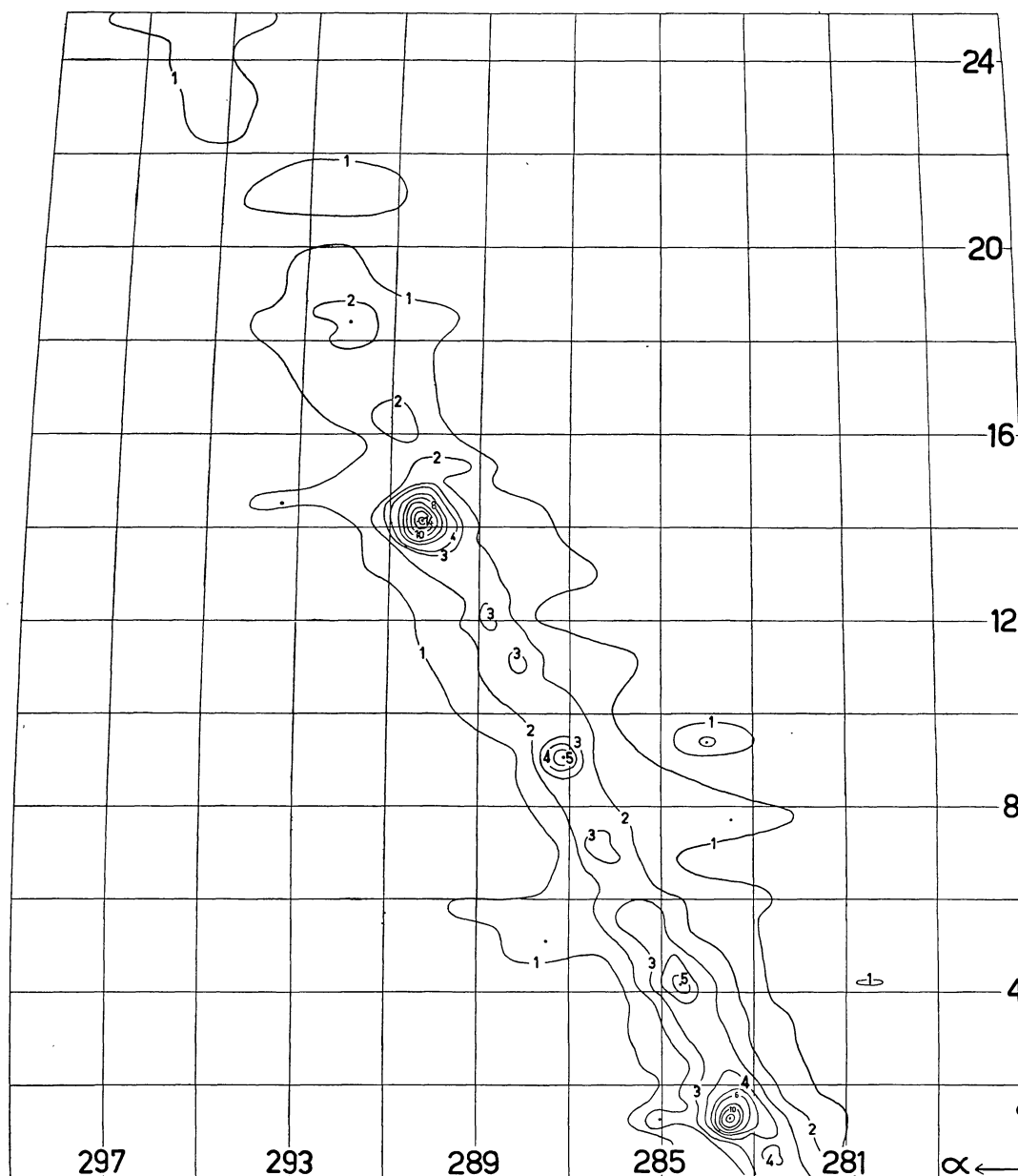
Map of region A in equatorial co-ordinates. Contour intervals are 5 units ( 3.25^\circ\text{K} in T_b ).
