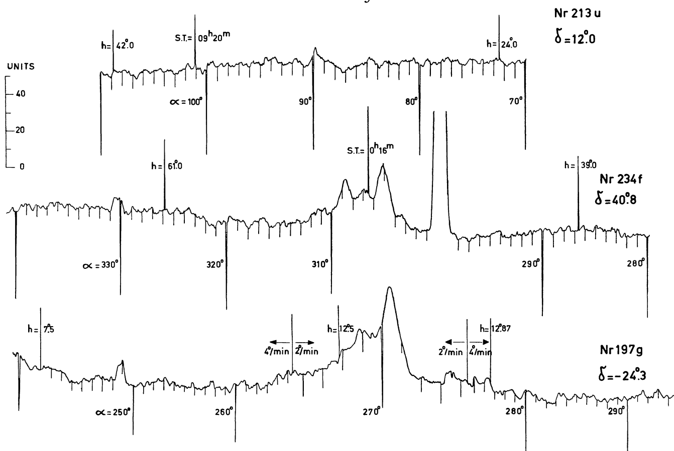
Sample recorder tracings of sweeps in \alpha , at constant \delta , for regions O, C and S.
