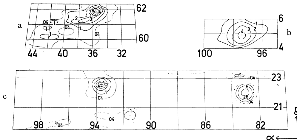
Maps of the surroundings of three discrete sources. Contour intervals are 5 units ( 3.25^\circ\text{K} in T_b ). a: IC 1795 (Nos 3, 4 and 5). b: Rosette nebula (No. 16). c: Crab nebula (Nos 9, 11, 13, 14 and 15).
