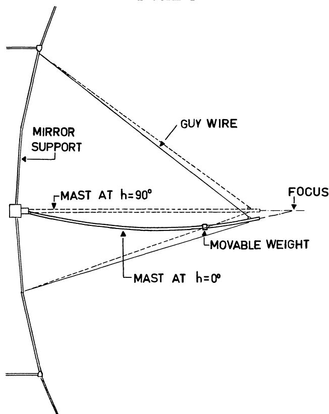
Suspending and bending of the antenna mast.
