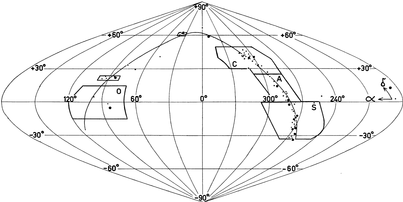
Equal-area chart of the whole sky, with the boundaries of the main survey and the two source maps, and the positions of the discrete sources. Big dots are sources with I > 30 units.
