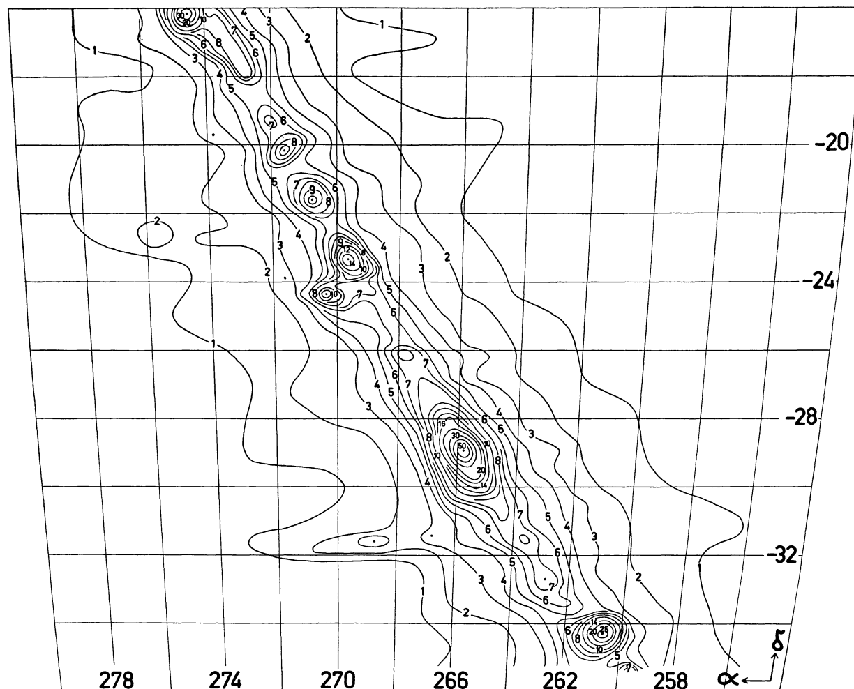
Map of region S (2) in equatorial co-ordinates. Contour intervals are 5 units ( 3.25^{\circ}\text{K} in T_b ).
