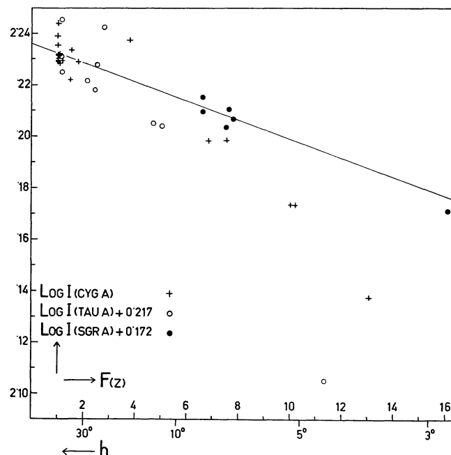
Intensities of three bright sources as a function of equivalent air mass, for determination of extinction.
