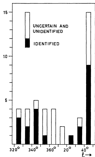
Number of sources, identified and unidentified or with uncertain identification, in 10-degree intervals in l .
