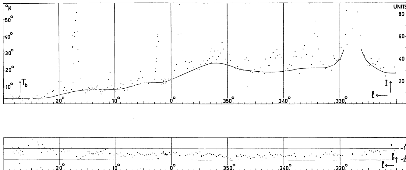
Intensity and latitude of the galactic ridge. Latitudes in the neighbourhood of bright sources (+) have been omitted.
