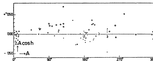
Deviation \Delta A \cos h from the standard position of radio stars.
