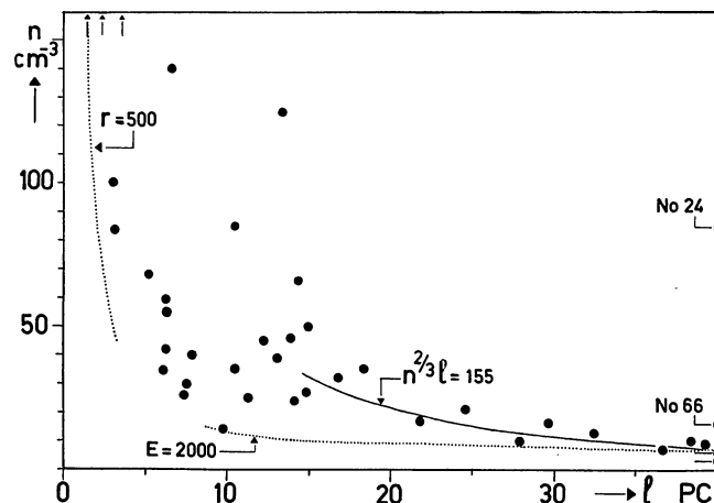
Density n of emission nebulae as a function of diameter l . Region to the left of and below the dotted lines is below the limit of detection.
