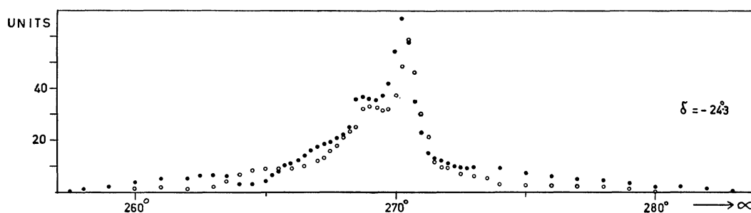
Example of a reduced cross-section.
