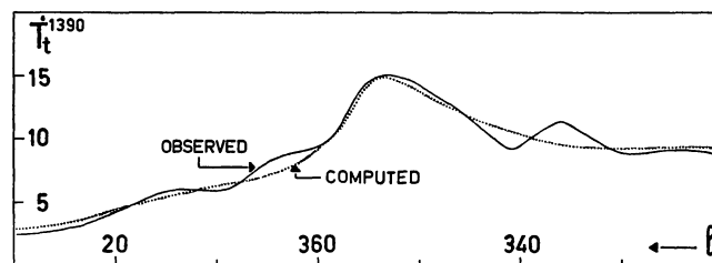
Observed and computed brightness temperatures of the thermal radiation along the galactic ridge.
