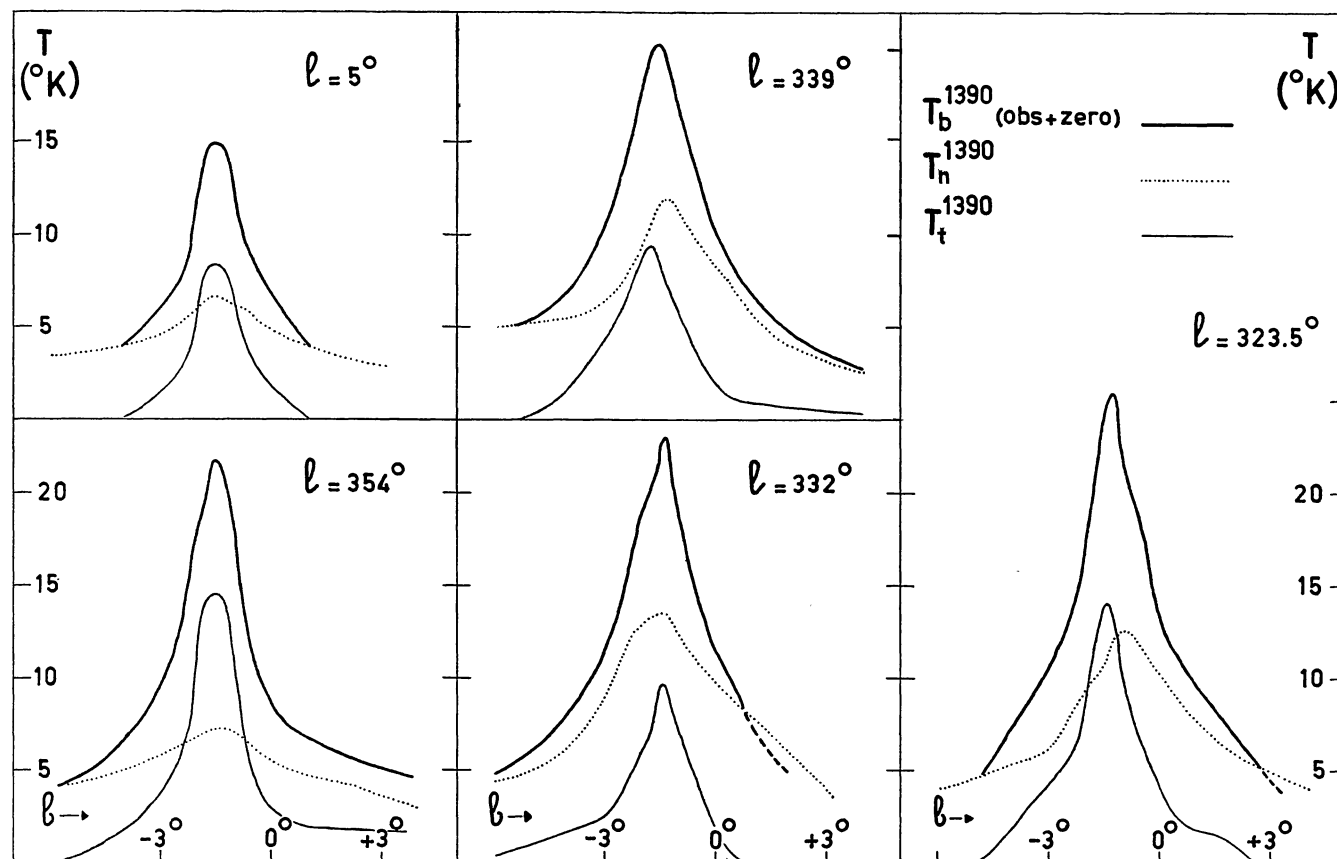
Total, thermal and nonthermal brightness temperatures in cross-sections perpendicular to the galactic plane, at 1390 Mc/s.
