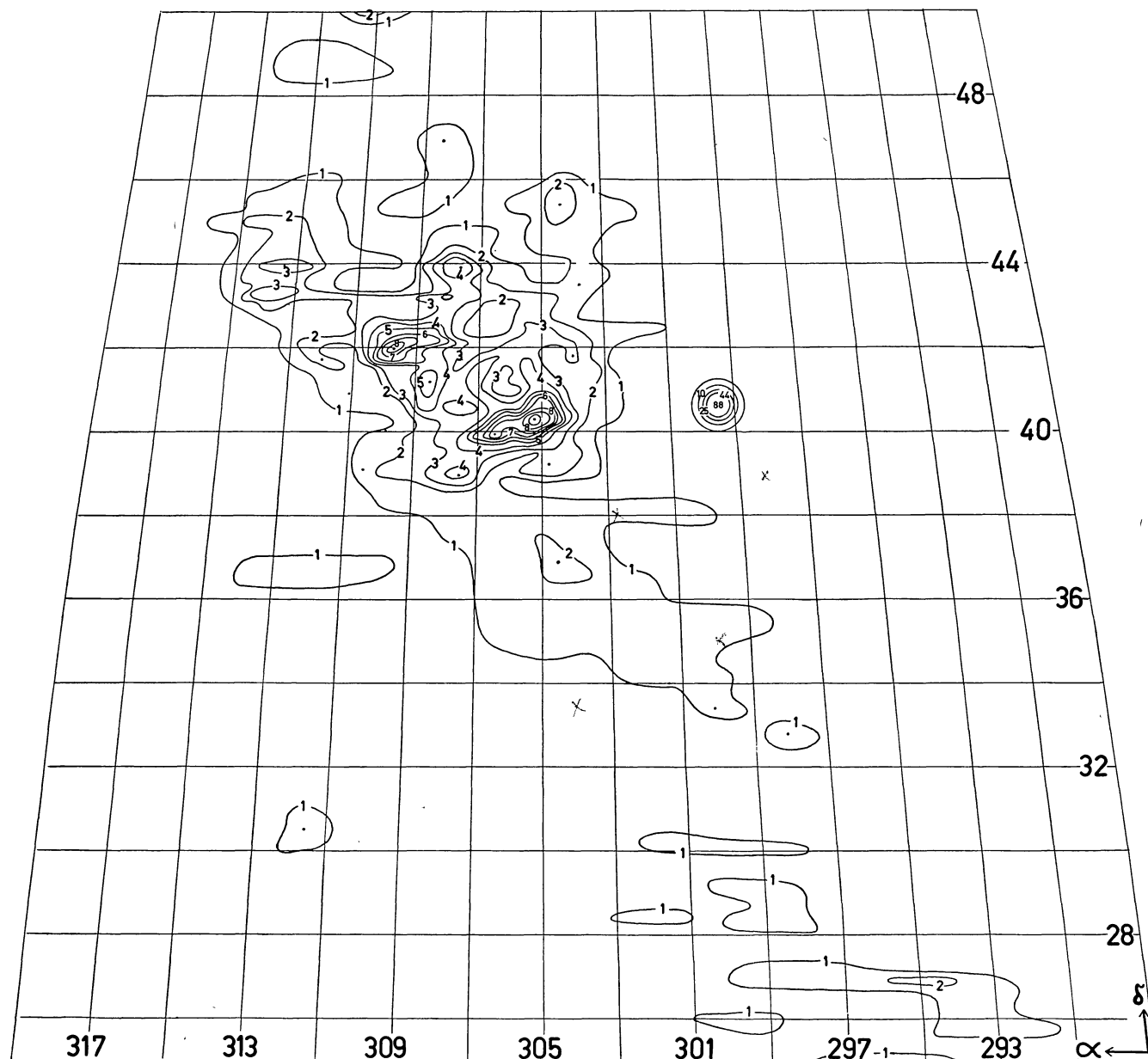
Map of region C in equatorial co-ordinates. Contour intervals are 5 units ( 3.25^\circ\text{K} in T_b ).
