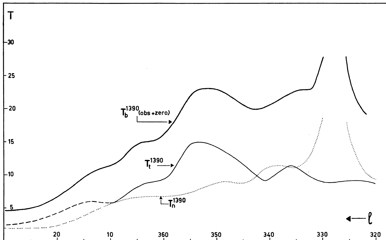
Total, thermal and nonthermal brightness temperatures along the galactic ridge, at 1390 Mc/s.
