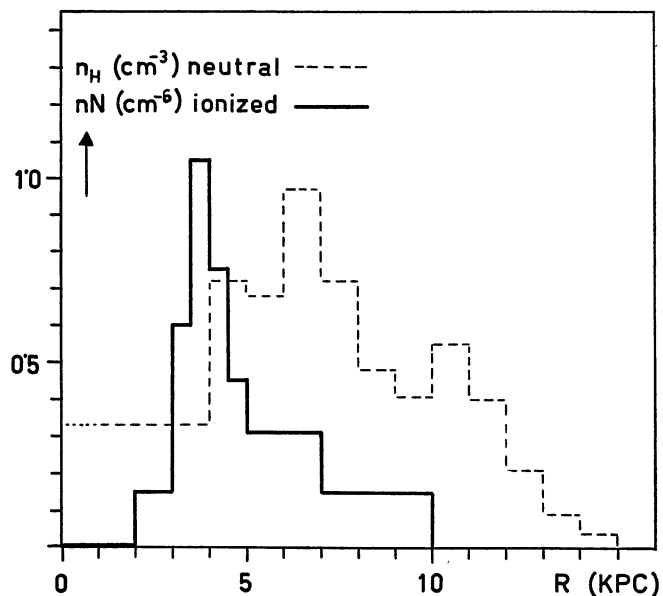
Density distribution of ionized and neutral hydrogen in the Galactic System. n = average space density, N = average density inside one cloud, assumed to be between 5 and 10 \text{ cm}^{-3} .
