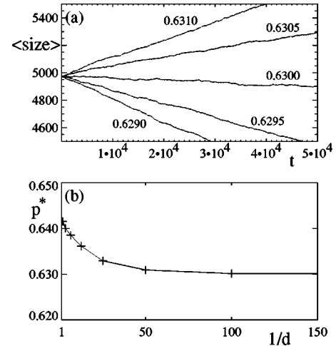
FIG. 19. (a) Time evolution of the average size of an active droplet (averaged over 500 realizations) of initial size 5000, for p = 0.631 , 0.6305 , 0.6300 , 0.6295 , and 0.629 . The slope of these curves varies linearly with p in this regime, yielding that the droplet starts to spread for p = 0.63012(4) . (b) Critical value of p , p^* , where front velocity changes direction as a function of the soliton lifetime 1/d , for c = 0.1 . The error bars are smaller than the symbol size. For d \searrow 0 , p^* \searrow 0.6298(2) , while for d = 1 , p^* approaches 0.6415(5) . This latter value is slightly different from the soliton-free value; even though d = 1 , solitons live for one time step and hence slightly alter the critical value.
