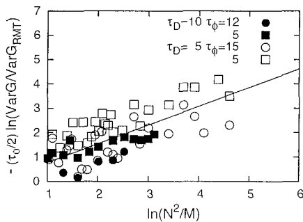
FIG. 3 Four data sets of fixed \tau_\phi , \tau_D each consisting of a range of M between 10^2 and 2 \times 10^4 plotted on a double-logarithmic scale. The solid line with slope 1/\lambda = 0.76 is the scaling predicted by Eqs. (5) and (6).
