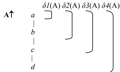
Figure 1: The ordering of degree functions
