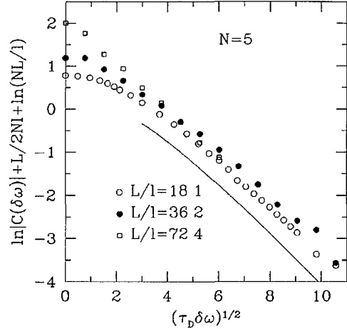
FIG. 1 Frequency dependence of the logarithm of the absolute value of the correlator C(\delta\omega) . The data points follow from a numerical simulation for N=5 , the solid curve is the analytical high-frequency result (6) for N \gg 1 (with \beta=1 ). The decay of the correlator is given by the diffusive time constant \tau_D = L^2/D even if the length L of the waveguide is greater than the localization length \xi = 6l . The offset of about 0.6 between the numerical and analytical results is probably a finite- N effect.
