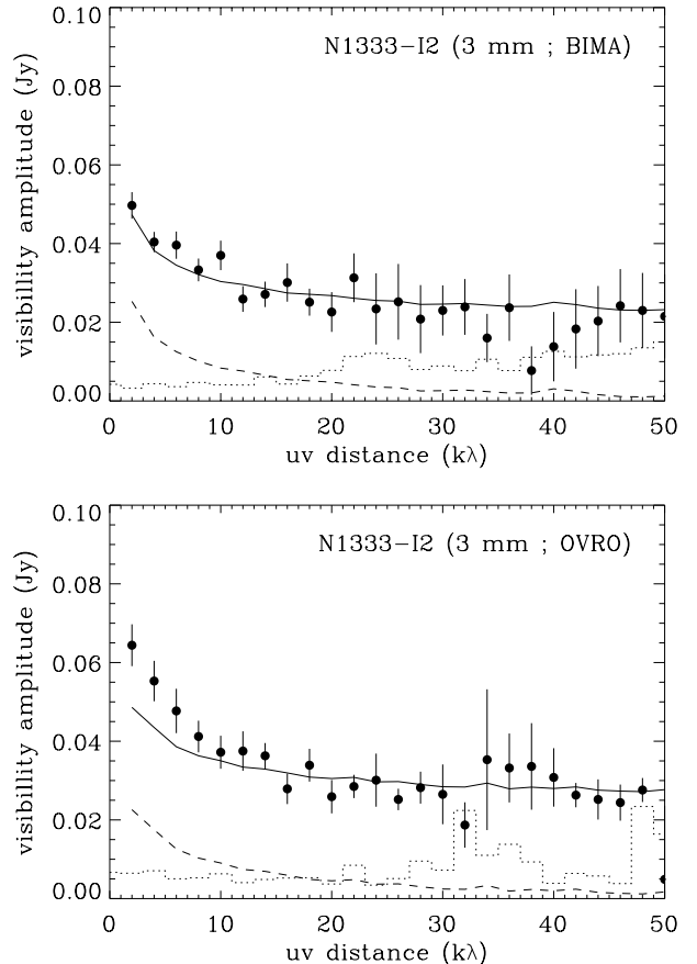
Fig. 3. Visibility amplitudes of the observed continuum emission from the BIMA ( upper panel ) and OVRO ( lower panel ) observations as a function of projected baseline length in k\lambda centered at the position of IRAS2A. The data are plotted as filled symbols with 1\sigma error bars, the continuous lines indicate the predictions from the continuum model of Paper I with the same (u, v) sampling as the observations – respectively with (solid) and without (dashed) an unresolved compact source of 22 mJy added to the model. The dotted histogram indicates the zero-expectation level: the expected amplitude signal due to noise alone in the absence of source emission.
