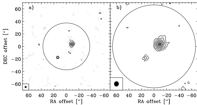
Fig. 2. Maps of continuum emission at 86–89 GHz from OVRO a) and BIMA b) . Offsets are with respect to the pointing center of \alpha(2000) = 03^{\text{h}}28^{\text{m}}56.29 and \delta(2000) = 31^{\circ}14'33.93 . Contours are shown at 3\sigma , 6\sigma , 12\sigma , 24\sigma and 48\sigma , where \sigma is the rms noise level of Table 3. The filled ellipses in the lower left corner of the panels indicate the synthesized beam sizes; the large circles show the 50% sensitivity levels of the primary beams.
