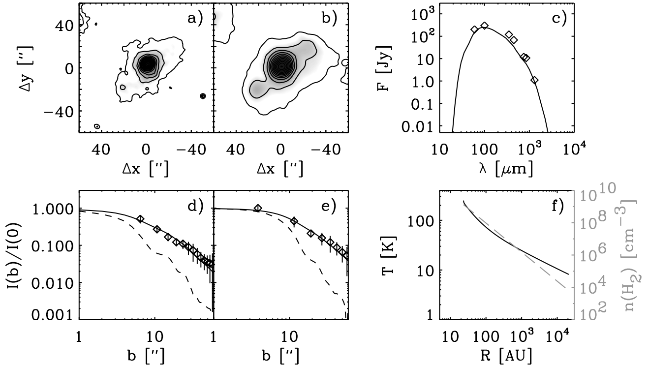
Fig. 1. a) and b) SCUBA maps of IRAS2 at 450 and 850 \mu\text{m} , respectively, centered on IRAS2A. c) Observed SED (symbols) and model fit (solid curve). d) and e) Brightness profiles at 450 and 850 \mu\text{m} (symbols) and the model fit (solid curve). The dashed curves show the beam profiles. f) Density (dashed line) and temperature (solid line) distributions of best-fit model. See Paper I for details.
