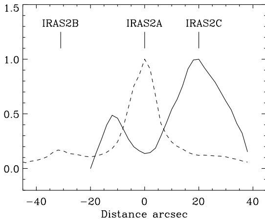
Fig. 13. The contrast between the N 2 H + and SCUBA emission: the N 2 H + emission divided by the 450 \mu m continuum emission (normalized) along a straight line with a position angle of 45° through IRAS2A (solid line) and the 450 \mu m continuum emission in the same positions (dashed line).
