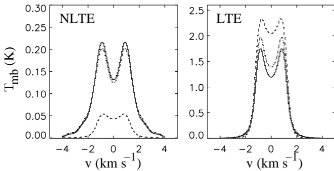
Fig. 11. Comparison of the CN 3–2 emission line for NLTE (left) and LTE (right) populations. The dash-dotted lines are for Spectrum A, the solid lines for Spectrum B, and the dashed lines for Spectrum C. The spectra have been convolved with a beam of 5.33''.
