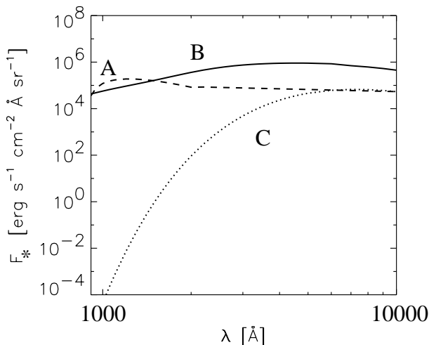
Fig. 6. Comparison of the mean intensity at a radius of R = 105 AU for the three stellar spectra: Spectrum A (dashed line), Spectrum B (solid line), and Spectrum C (dotted line) (see text).
