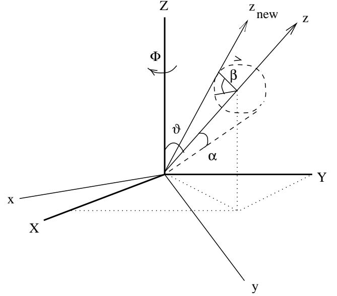
Fig. A.1. Scattering of a photon propagating in the direction (\phi, \theta) through angles \alpha and \beta . The new photon direction will lie on a cone defined by \alpha and \beta .
