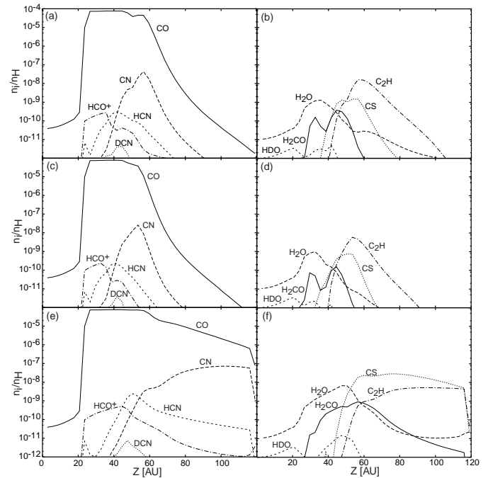
Fig. 7. Vertical distribution of molecules at R = 105 AU and t = 1 \times 10^6 yr. Panels a) and b) are for Spectrum A, panels c) and d) are for Spectrum B and panels e) and f) for Spectrum C.
