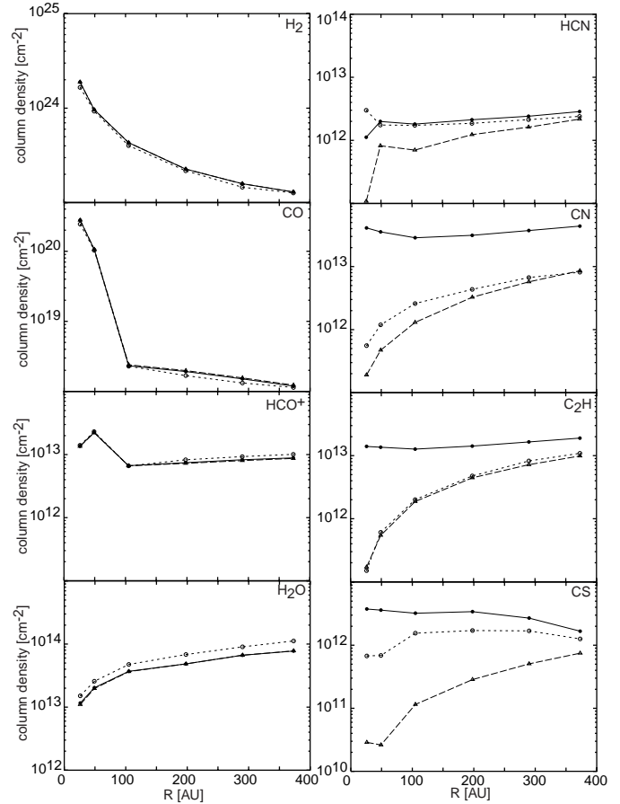
Fig. 5. Radial distribution of column densities at t = 1 \times 10^6 yr. The dashed lines with open circles refer to the A-2D model, the long-dashed lines with the solid triangles to the ND-2D model, and the solid lines with closed circles are for the full 2D model.
