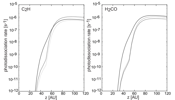
Fig. 3. Photodissociation rates of \text{C}_2\text{H} and \text{H}_2\text{CO} as functions of height from the midplane at R = 105 AU. Rates are calculated using the radiation field obtained via the full 2D Monte Carlo radiative transfer ( solid lines ). For comparison, rates obtained via the approximate 2D method adopting the depth-dependent function of van Dishoeek (1988) ( dotted lines ) and the new standard model ( dashed lines ) are shown.
