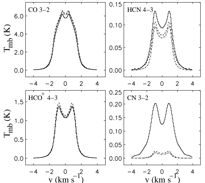
Fig. 9. Comparison of emission lines for the full-2D radiative transfer model (solid lines), the 2D radiative transfer model without CO and H 2 dissociation (ND-2D; dot-dashed) and the approximate 2D model (A-2D; dashed lines). The CO 3-2, HCO + 4-3, CN 3-2 and HCN 4-3 lines are convolved with a beam equal to the size of the source on the sky (5.33'').
