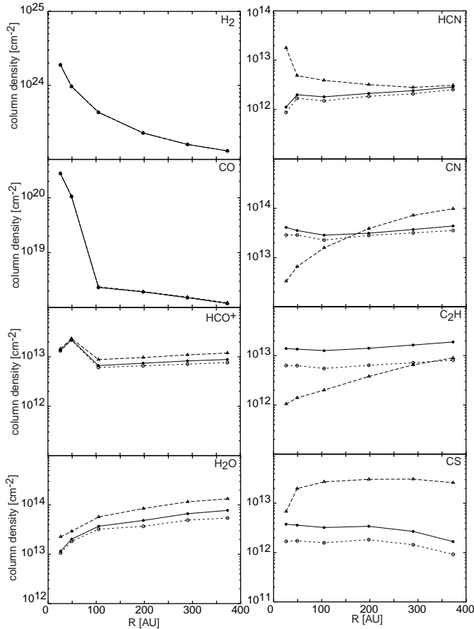
Fig. 8. Radial distribution of molecular column densities at t = 1 \times 10^6 yr. Solid lines with closed circles are for Spectrum A, dashed lines with open circles for Spectrum B, and long-dashed lines with triangles for Spectrum C.
