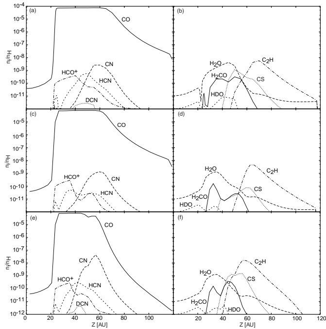
Fig. 4. Vertical distribution of molecules at R = 105 AU and t = 1 \times 10^6 yr. In panels a ) and b ), the approximate-2D (A-2D) method is adopted with the depth-dependent dissociation rates. The dissociation rates used in panels c ) and d ) are determined using the full 2D radiative transfer (ND-2D). In both cases the stellar UV is assumed not to be energetic enough to dissociate H_2 and CO. In panels e ) and f ), dissociation rates are determined using the full 2D radiative transfer, and dissociation of H_2 and CO via the stellar UV is considered.
