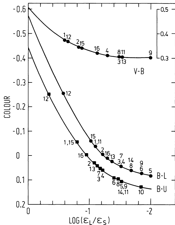
Fig. 2. Determination of the contamination \varepsilon_L/\varepsilon_s by line emission, see Sect. I. Left hand scale for B-L and B-U , right hand scale for V-B . Observations are indicated by solid dots and squares. Coincidences are not shown for values \varepsilon_L/\varepsilon_s < 0.01
