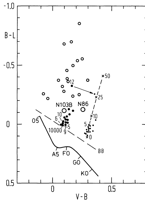
Fig. 3. Two colour diagram. Large solid dots: reddening corrected ( A_{VJ} = 1.4 ) colours of M1, small dots: observations of M1; dashed line: relation of Eq. (3) for values \varepsilon_L/\varepsilon_s \times 100 as indicated; open circles: reddening corrected observations of other SNR (Paper II). Black body (BB) line and main sequence line are shown
