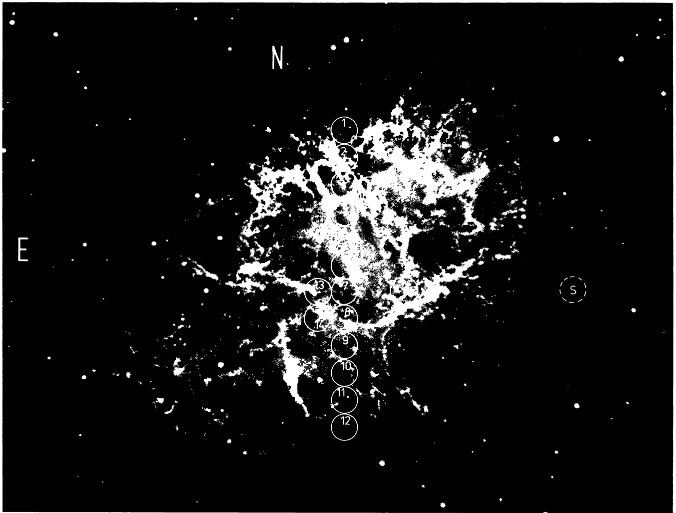
Fig. 1. Distribution of filaments of M 1, line emission of H_\alpha and [N II] (taken from Baade, 1956), and positions of observations. The dashed circle gives the sky background
