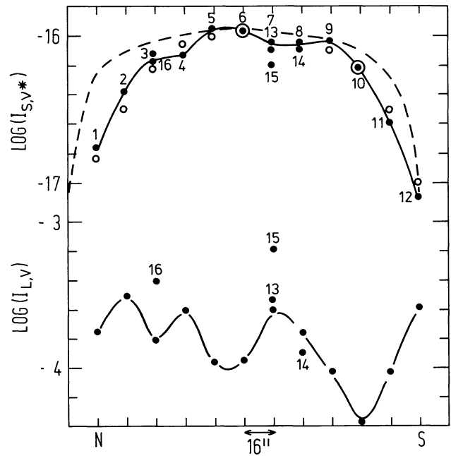
Fig. 4. Absolute intensities derived from V passband fluxes, corrected for A_{VJ}=1^m4 . The upper curves give the intensity I_{S,\nu^*} of the synchrotron radiation for the frequency \nu^*=5.56 \cdot 10^{14} \text{ Hz} at the center of V passband, intensity in \text{erg cm}^{-2} \text{ s}^{-1} \text{ Hz}^{-1} \text{ sterad}^{-1} . Solid dots: derived from observations of this paper, open circles: taken from Woltjer (1957) and normalized to the intensity at position 6; dashed line: emission of a homogenous, optically thin sphere. Lower curve: line intensity I_{L,\nu} received in V passband, in \text{erg cm}^{-2} \text{ s}^{-1} \text{ sterad}^{-1} .
