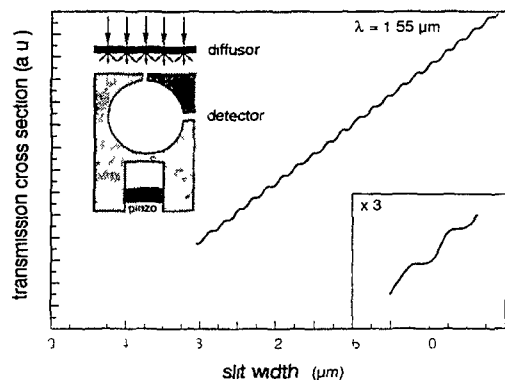
Figure 12 Experimental demonstration of equidistant steps in the transmission cross-section of a slit of adjustable width. A 2D Lambertian monochromatic source is obtained by illuminating a diffusor consisting of a random array of parallel fibers by a diode laser beam. An integrating sphere is used to obtain a detector signal proportional to the transmission cross-section. [From Montie et al. [23]]
