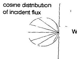
Fig. 11. An isotropic velocity distribution in a wide region of an electron gas in thermal equilibrium causes a \cos \theta distribution of the flux incident on a narrow slit. \theta is the angle with respect to normal incidence. The magnitude of the flux is indicated by straight lines for various angles of incidence.
