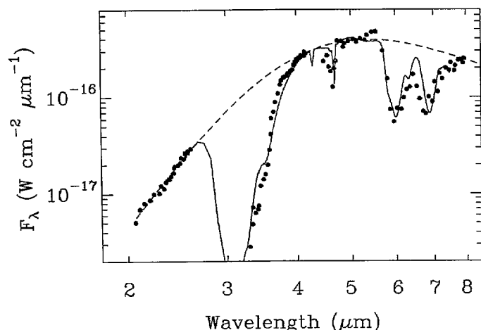
FIG. 2.—The original 2\text{--}8 \mu\text{m} spectrum of W33A (Soifer et al. 1979) compared with a composite spectrum of irradiated \text{H}_2\text{O}/\text{NH}_3/\text{CO}/\text{O}_2 = 10/1/1 . The IR spectrum taken after 20 hr annealing time at 176 K was multiplied by a factor of 12 and added to the IR spectrum taken after simultaneous irradiation and deposition at 12 K. The resolution is 4 \text{ cm}^{-1} . The continuum is taken from Fig. 2 in Baas et al. (1988).
