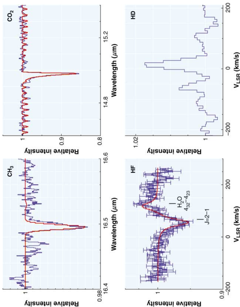
Figure 5 New gas-phase molecules detected by ISO . The red line in each panel indicates the model spectrum. CH 3 v 2 Q-branch toward Sgr A* ( top left ) (Feuchtgruber et al. 2000); CO 2 v 2 band toward AGFL 2136 ( top right ) (van Dishoeck et al. 1996, Boonman et al. 2003b); HF J = 2 - 1 toward Sgr B2 ( bottom left ) (Neufeld et al. 1997); HD J = 1 - 0 line toward the Orion Bar ( bottom right ) (Wright et al. 1999).
