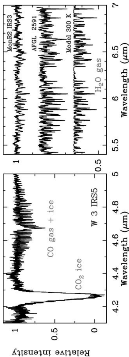
Figure 4 Normalized SWS spectra toward massive protostars showing absorption by various species: CO 2 v 3 and CO v 1 bands ( left panel ) and H 2 O v 2 band ( right panel ). The spectra in the right panel have been shifted vertically for clarity. Gas-phase molecules show sharp unresolved rovibrational lines in a characteristic pattern, whereas ices have a single broad absorption (Based on van Dishoeck 1998, Helmich et al. 1996, and Boonman & van Dishoeck 2003c).
