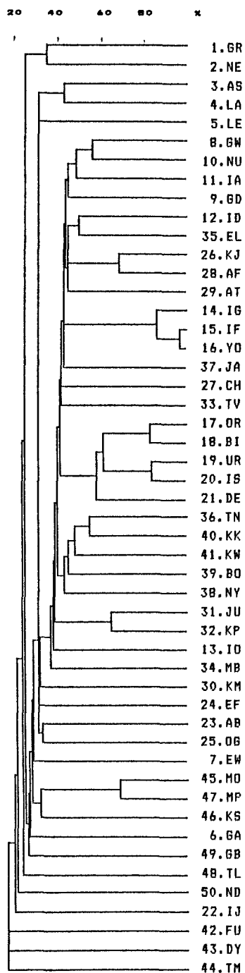
Figure 2: NN Subclassification
