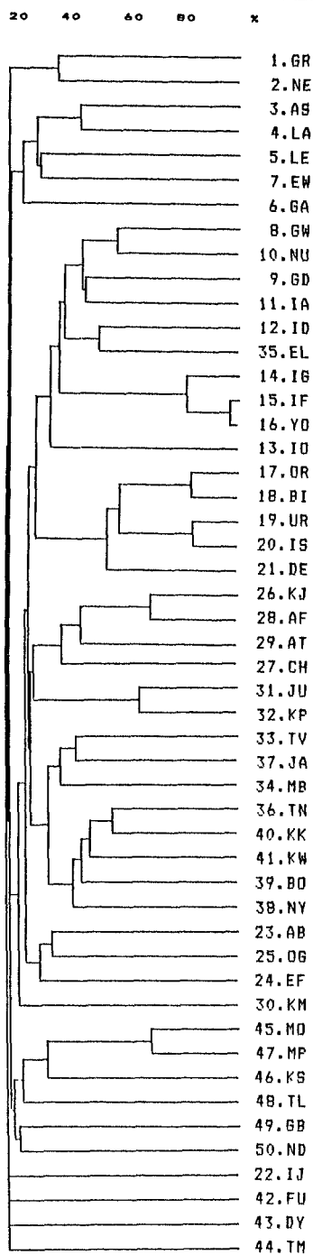
Figure 1: BA Subclassification
