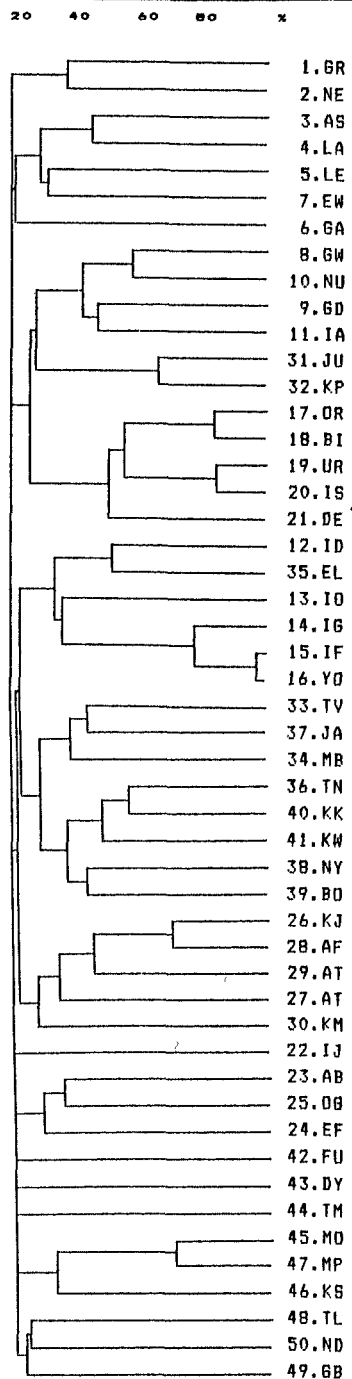
Figure 3: FN Subclassification
