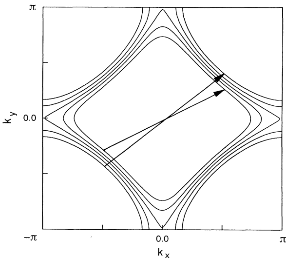
FIG. 2. Fermi surface at different doping levels x - x_{vh} = -0.10, -0.05, 0.00, 0.05 , and 0.12 for \epsilon = 1.2 eV, t = -1.5 eV, and t' = 0.5 eV. The arrows mark the direction of “best” nesting.
