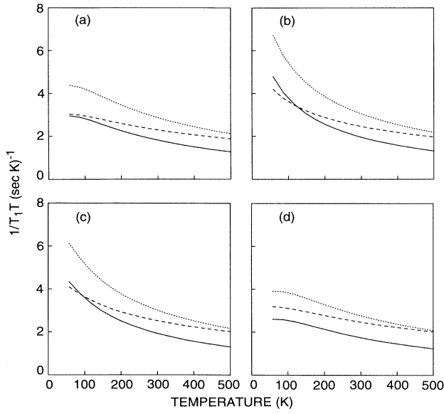
FIG. 9. Calculated NMR relaxation rates (T_1 T)^{-1} corresponding to the hyperfine coupling constants in Fig. 8. Band parameters are the same as Figure 4(a)–4(d). Solid line (^{63}T_1^{-1})_{\parallel} ; dotted line (^{63}T_1^{-1})_{\perp} ; dotted line ^{17}T_1^{-1} \times 10 . Note that the oxygen relaxation rate has been scaled by a factor of 10.
