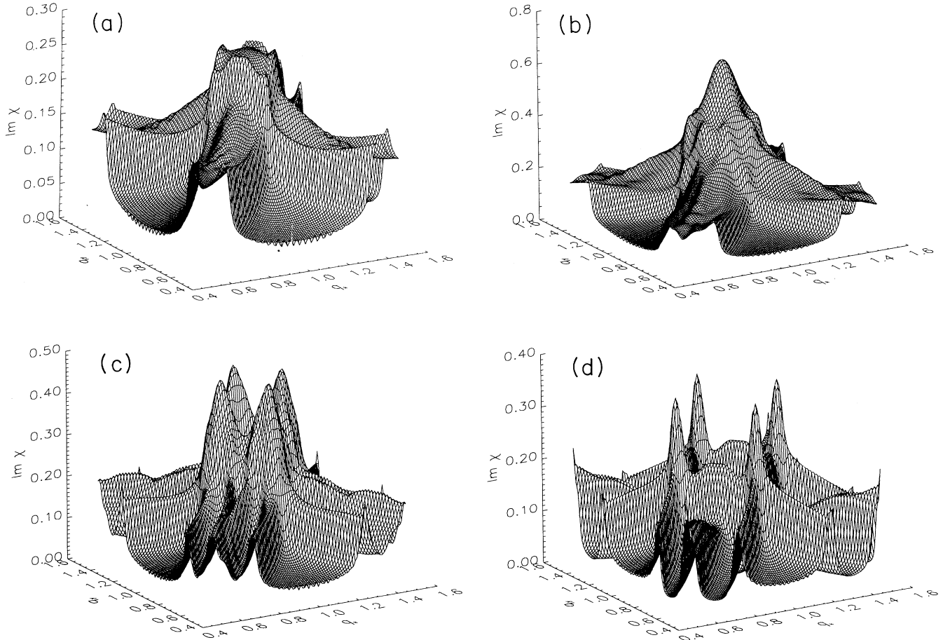
FIG. 4. Perspective plot of \text{Im}[\chi(\mathbf{q}, \omega = 2 \text{ meV})]/\mu_B^2 convoluted with a Gaussian broadening (see text) for \varepsilon = 1.2 \text{ eV} , t = -1.5 \text{ eV} , t' = 0.5 \text{ eV} , \lambda = 0.3 , \omega_c = 1 \text{ eV} , T = 2 \text{ meV} , and m^* = 5 . Contour labels are values in (\text{eV})^{-1} . The dashed lines mark lines of singularities for FS “touching”. Doping levels are x - x_{\text{vh}} = -0.04 (a); 0.01 (b); 0.06 (c); 0.12 (d).
