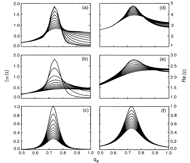
FIG. 11. Susceptibility \text{Im}[\chi(q=\pi(1, q_x)), \omega=2 meV] [left panels, (a)–(c)] and \text{Re}[\chi(q=\pi(1, q_x)), \omega=0] [right panels, (d)–(f)] for a FL (a)–(d), MFL (b), (e), and AFL (c), (f), for a set of temperatures T=0.002, 0.005, 0.010, 0.015, \dots, 0.050 eV. For the FL and MFL, parameters are \varepsilon=1.2 eV, t=-1.5 eV, t'=0.5 eV, m^*=5 , with \omega_c=1 eV, \lambda=0.3 (MFL) and \text{Im}(\Sigma)=2 meV (FL). For the AFL, the susceptibility is described by Eq. (6), and we used \xi(T)^{-2} = \xi_0^{-2}(1 + T/T_0) with \pi\xi_0=15 and T_0=0.05 eV.
