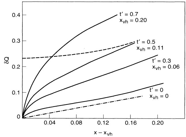
FIG. 3. Position of dominant peaks in \chi''(\mathbf{q}, \omega \rightarrow 0) , at \mathbf{Q}_s = \pi(1 - \delta Q, 1) as a function of doping measured from x_{vh} , for \epsilon = 1.2 eV, t = -1.5 eV, and several values of t' . In the case of t' = 0.5 eV only, the position of the secondary nesting peak is shown by the dashed line. The chain line is expected from a model of domain walls separating AF regions.
