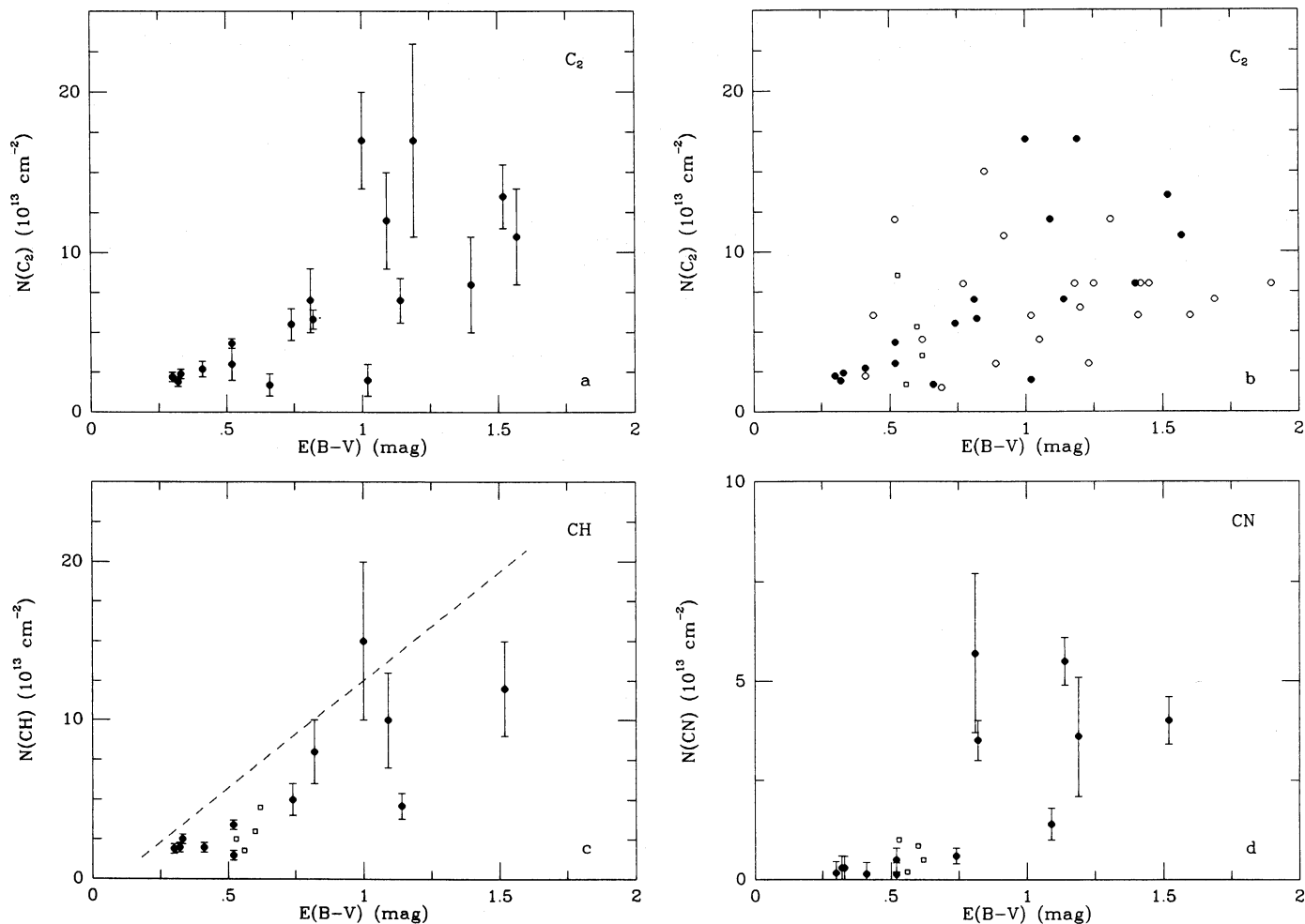
FIG. 8.—Molecular column densities as functions of extinction. (a) C 2 vs. E(B-V) for lines of sight with detected C 2 . (b) C 2 vs. E(B-V) for all lines studied in this work. Filled circles denote lines of sight with detected C 2 ; open circles refer to upper limits. Open squares indicate the C 2 column densities measured by Federman and Lambert (1988) for lines of sight in Cepheus. (c) CH vs. E(B-V) for lines of sight studied in this paper. The open squares indicate the column densities measured for stars in Cepheus by Chaffee and Dunham (1979) and Federman and Lambert (1988). The dashed line is the relation found by Mattila (1986) for dark clouds. The one point lying above this line refers to HD 29647. (d) CN vs. E(B-V) for lines of sight studied in this work. Open squares indicate the CN column densities in the Cepheus region based on measurements by Chaffee and Dunham (1979), Joseph, Snow, and Seab (1988) and Federman and Lambert (1988).
