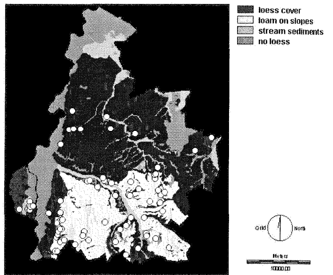
Figure 2. The distribution of loess and the location of the Middle Palaeolithic sites.
