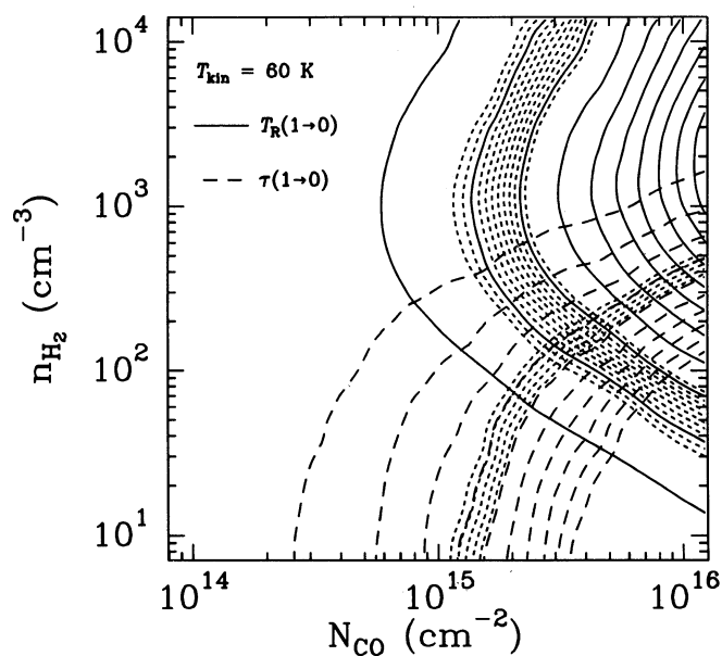
FIG. 2.—Contour plots of 12 CO 1–0 emission (solid line) and line center optical depth (long-dashed line) as functions of 12 CO column density and H 2 number density for T_{\text{kin}} = 60 K. Contour levels are T_R = 1.0, 2.0, \dots , K, and \tau = 0.3, 0.6, \dots, 3.0 . Observed values are indicated with their respective errors by the short-dashed lines. For the lowest temperature consistent with the observations, T_{\text{kin}} = 20 K, the inferred n_{\text{H}_2} is enhanced by about a factor of 2.
