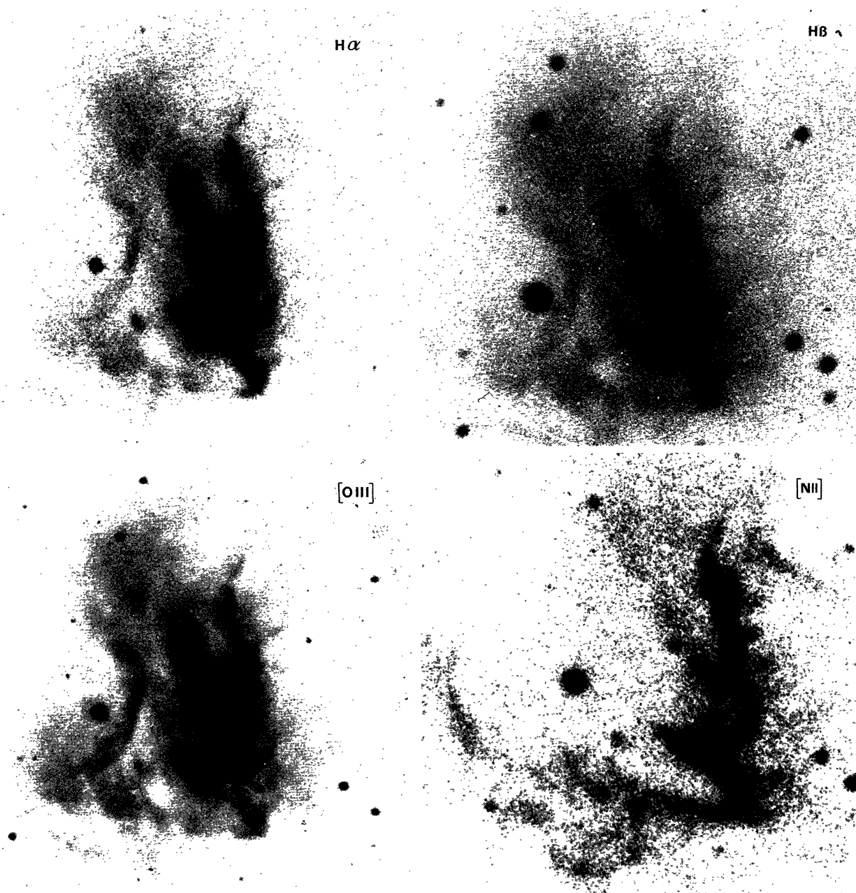
Fig. 1. Monochromatic photographs of S 206. The H\beta photograph was taken by M. C. Lortet
