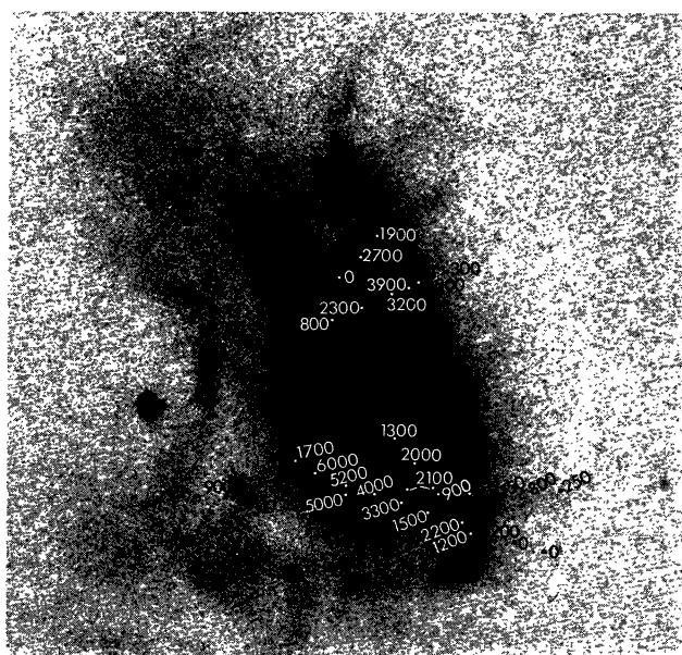
Fig. 7. Electron densities obtained from optical observations
