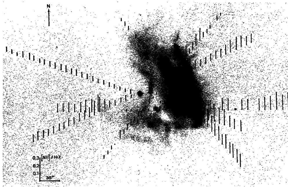
Fig. 6. Variations of the [\text{N II}]/\text{H}\alpha ratio over the field of the nebula; the foot of each segment indicates the point where the measure has been done; the size of the segments is proportional to the [\text{N II}]/\text{H}\alpha ratio
