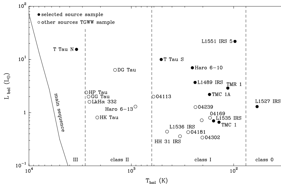
FIG. 10.—Diagram of bolometric luminosity against bolometric temperature (BLT diagram) of the TGWW source sample. The objects studied in the present paper are indicated by the filled symbols. The main sequence is located at the extreme left of the plot.
