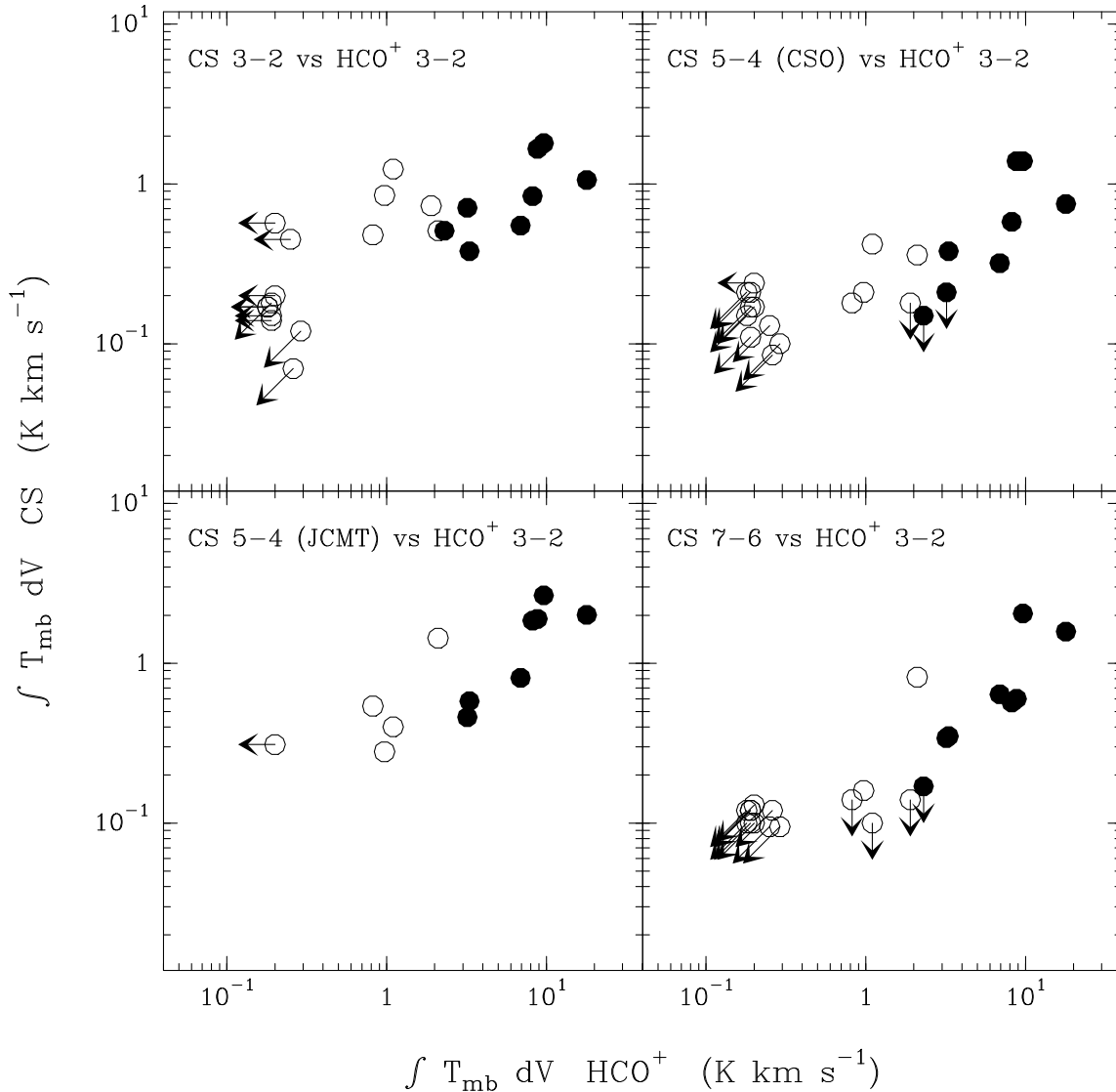
FIG. 7.—Integrated intensity in CS 3–2, 5–4 (CSO and JCMT), and 7–6 (from Moriarty-Schieven et al. 1995) against \text{HCO}^+ 3–2 for the TGWW source sample. The nine objects investigated in the present paper are indicated by the filled symbols. The size of the symbols corresponds to the uncertainty in the data.
