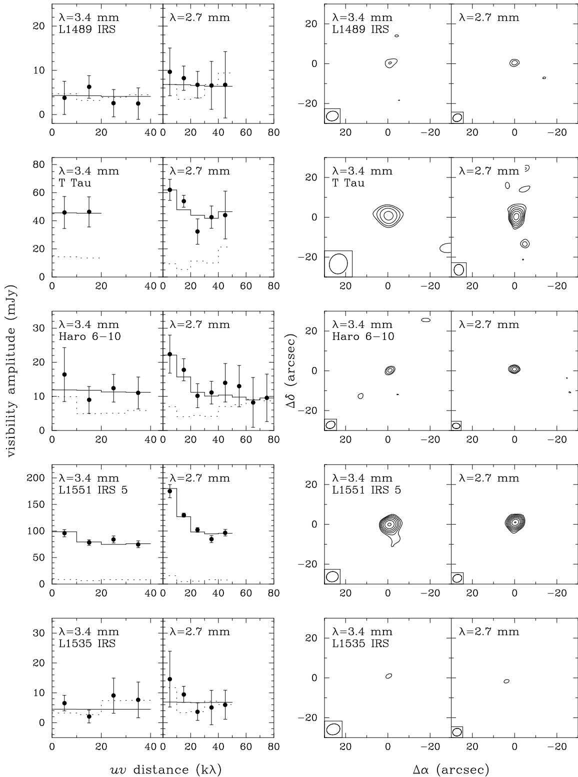
FIG. 2.—In the left-hand panels the vector-averaged, u - v -binned 3.4 and 2.7 mm visibility amplitudes in mJy are plotted against u - v separation in k\lambda . The observations, indicated by the filled symbols, are shown with their 1\sigma error bars. The dotted line is the zero-signal expectation value, the thick solid line a model fit (see § 4.1, Table 4). In the right-hand panels the cleaned images of the 3.4 and 2.7 mm continuum emission are shown, using natural weighting. The beam sizes are indicated in the lower left-hand corner of each panel. The contour levels start at 2\sigma ( \approx 3 mJy beam ^{-1} ; except for T Tau: \sim 10 mJy beam ^{-1} at 3.4 mm, \sim 6 mJy beam ^{-1} at 2.7 mm) and increase in steps of 2\sigma .
