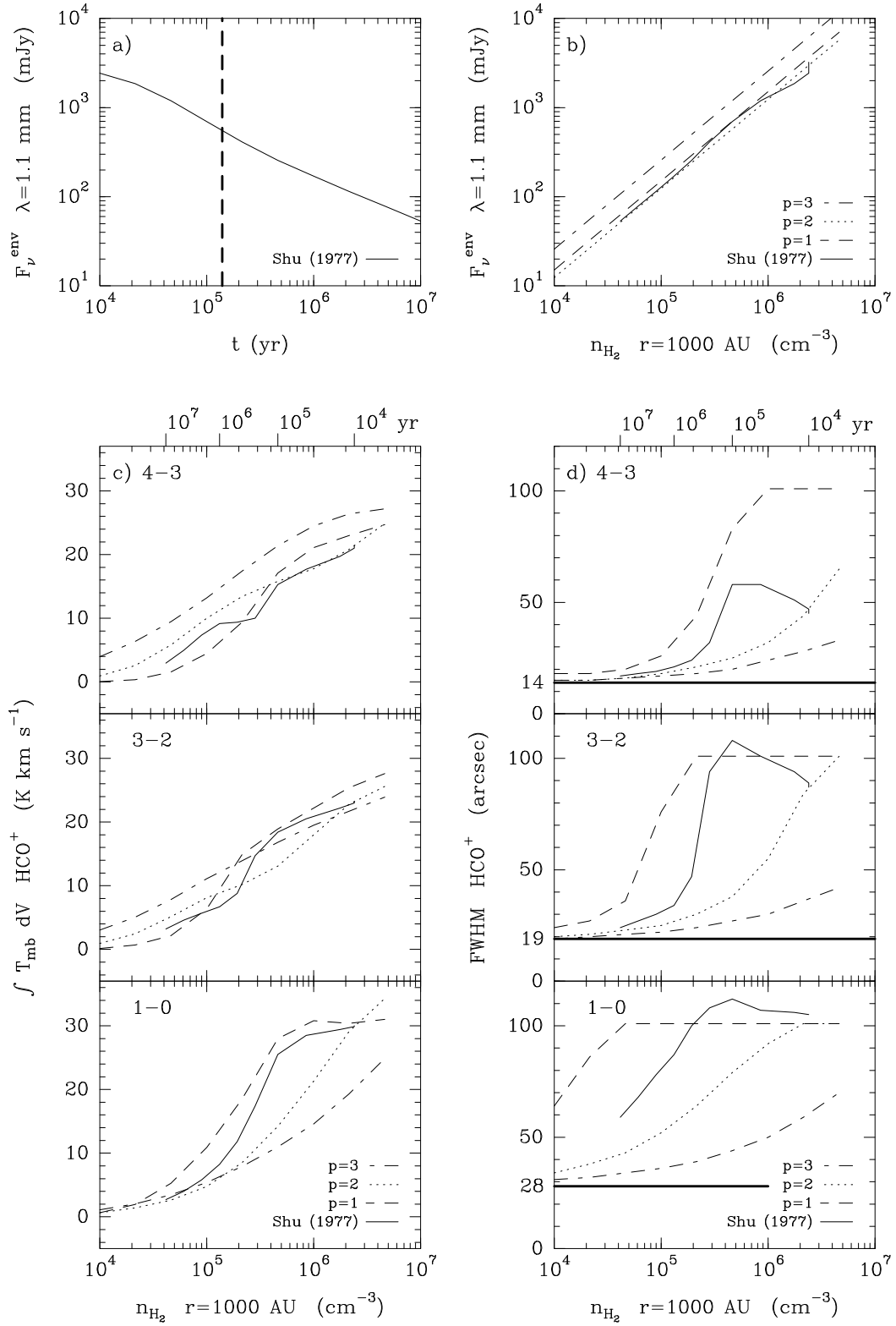
FIG. 6.—(a) Continuum flux at 1.1 mm in mJy as function of postcollapse time in yr for the Shu (1977) collapse model. The time at which the collapse expansion wave reaches the outer boundary of the model core is indicated by the dashed line. (b) 1.1 mm flux in mJy as function of \text{H}_2 number density at an arbitrary radius of 1000 AU, for the Shu (1977) collapse model and three power-law density distributions with slopes of p = 1, 2 , and 3. (c) Integrated intensity of \text{HCO}^+ 4-3 (top), 3-2 (middle), and 1-0 (bottom), in \text{K km s}^{-1} , as functions of density at 1000 AU for the same models, assuming a constant \text{HCO}^+ abundance of 1.2 \times 10^{-8} . (d) FWHM source size, after beam convolution, for \text{HCO}^+ 4-3 (top), 3-2 (middle), and 1-0 (bottom) as functions of density at 1000 AU for the same models. The respective beam sizes are indicated by the thick horizontal lines.
