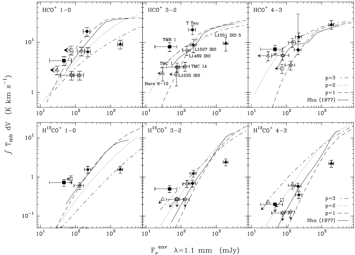
FIG. 5.—Integrated \text{HCO}^+ (top panels) and \text{H}^{13}\text{CO}^+ (lower panels) 1–0 (left column), 3–2 (middle column), and 4–3 (right column) emission as functions of 1.1 mm envelope flux. The objects of our sample are indicated by the symbols, together with error bars corresponding to the \sim 30\% calibration uncertainty. The error bar for T Tau in the \text{HCO}^+ 4–3 panel also contains the large contribution from the outflow to the line wings. Curves are drawn for the three power-law models and for the Shu (1977) collapse model. In the \text{HCO}^+ 3–2 panel the objects are identified, for comparison with Fig. 8.
