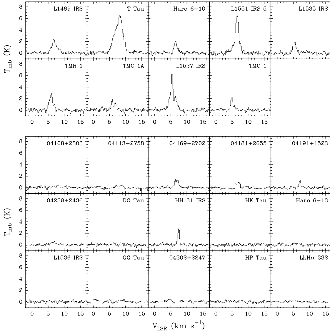
FIG. 1.— \text{HCO}^+ 3–2 spectra of the sources defined by Tamura et al. (1991) as YSOs (see Table 2). The nine strongest objects selected for further study are shown in the top panel; the others are shown in the lower panel. The vertical scale is antenna temperature T_{\text{mb}} in K, the horizontal scale is velocity V_{\text{LSR}} in \text{km s}^{-1} . The estimated calibration uncertainty of these \text{HCO}^+ 3–2 spectra is at least 30%, as discussed in § 3.2.
