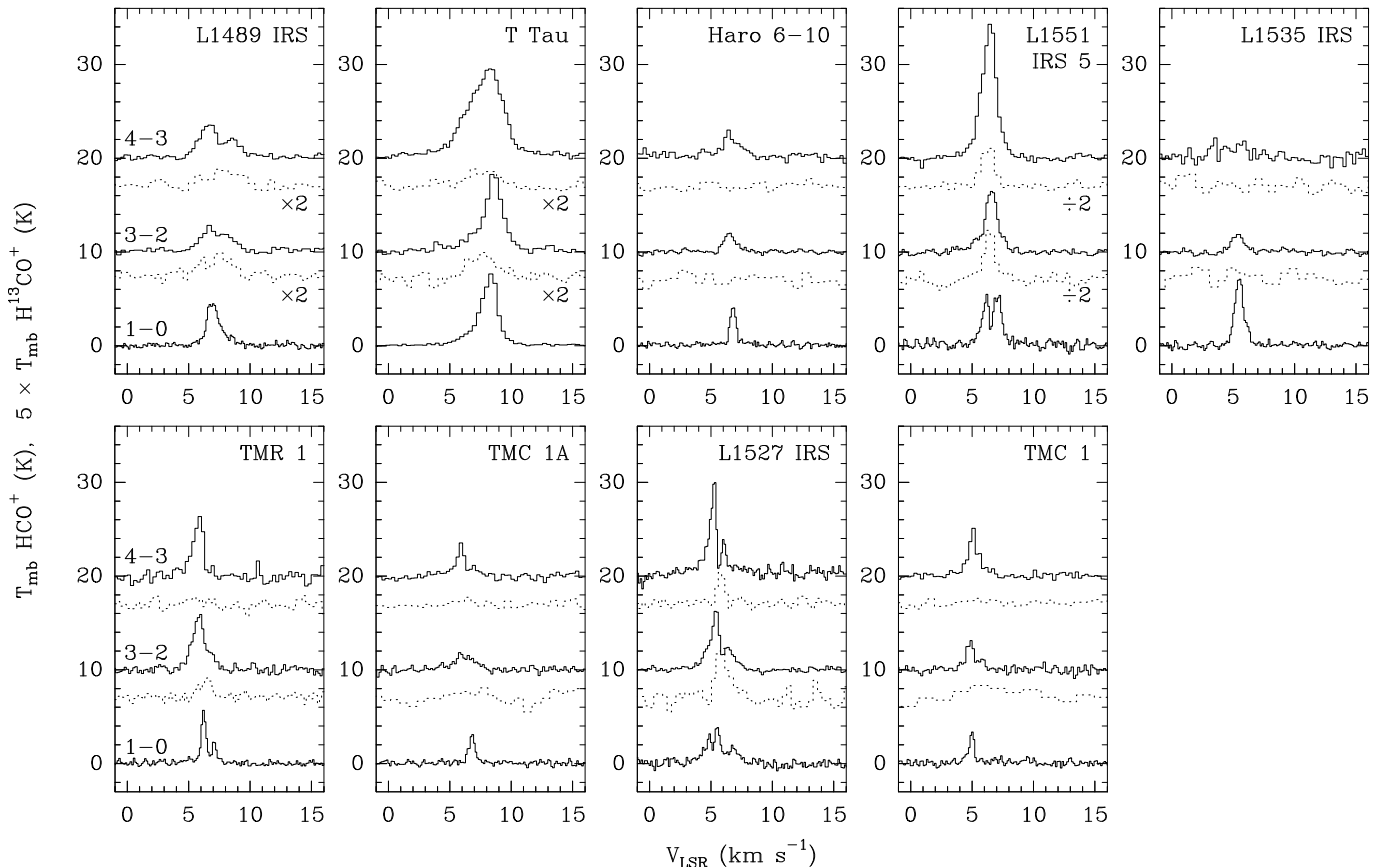
FIG. 3.—Spectra of \text{HCO}^+ 1–0 (bottom curves), 3–2 (middle curves), and 4–3 (top curves) toward the nine YSOs of our sample (solid lines). The \text{H}^{13}\text{CO}^+ 3–2 and 4–3 spectra are indicated by the dotted lines. The 3–2 and 4–3 spectra are offset by 10 and 20 K, respectively; the \text{H}^{13}\text{CO}^+ spectra have been multiplied by a factor of 5 (factor of 10 for L1489 IRS and T Tau; factor of 2.5 for L1551 IRS 5, as indicated). The vertical scale is antenna temperature T_{\text{mb}} in K, the horizontal scale is velocity V_{\text{LSR}} in \text{km s}^{-1} .
