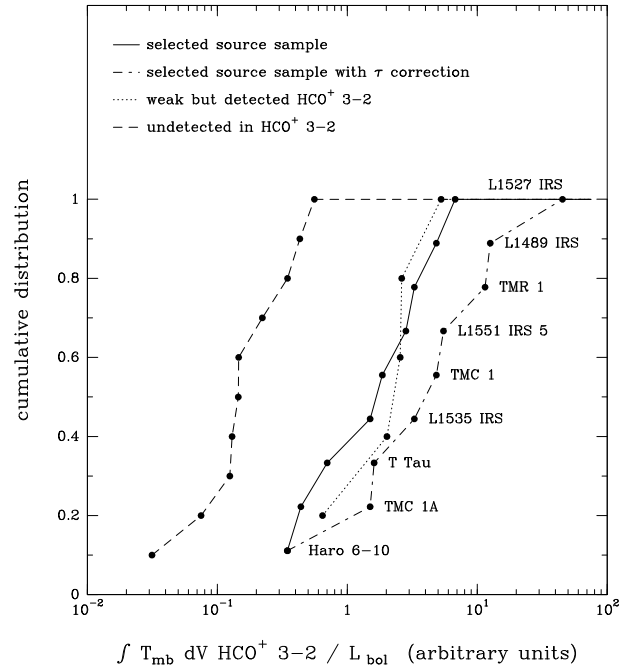
FIG. 9.—Cumulative distribution of \int T_{\text{mb}} dV(\text{HCO}^+ 3-2)/L_{\text{bol}} of the selected source sample (with and without correction for line opacity), those sources in the TGWW sample that are weak in \text{HCO}^+ 3–2, and the sources undetected in \text{HCO}^+ 3–2. The sources in the selected sample are identified along the \tau -corrected curve. The quantity \int T_{\text{mb}} dV(\text{HCO}^+ 3-2)/L_{\text{bol}} traces M_{\text{env}}/M_* , i.e., the relative evolutionary phase of an embedded object. Relatively young sources are located on the right of the plot, more evolved ones on the left.
