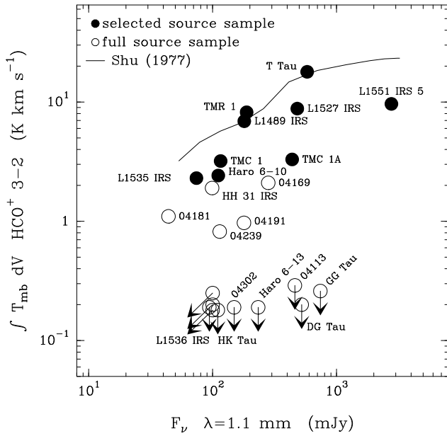
FIG. 8.—Integrated \text{HCO}^+ 3–2 against 1.1 mm single-dish flux for the full source sample. The nine objects investigated in the present paper are indicated by the filled symbols. The size of the symbols reflects the uncertainty in the data. Note that, in contrast with the fluxes used in Fig. 5, no correction is made for the contribution of any compact disks. For reference, the curve corresponding to the Shu (1977) collapse model is plotted.
