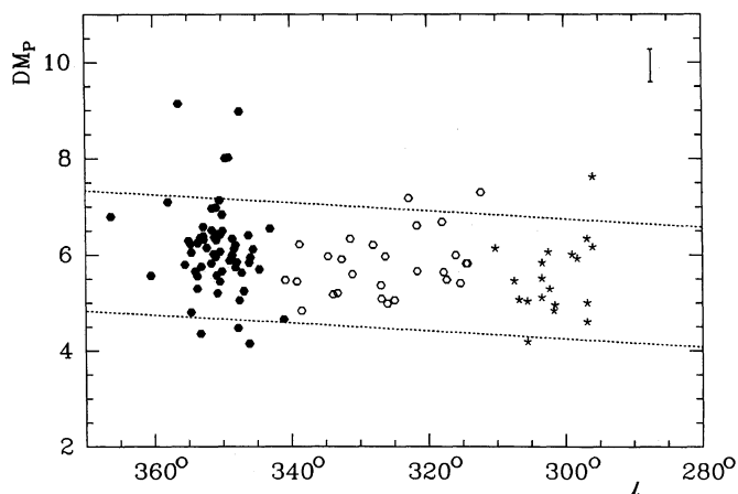
Fig. 9. Distance modulus as a function of galactic longitude for the established member-stars of the three subgroups. \bullet : Upper-Scorpius; \circ : Upper-Centaurus Lupus; * : Lower-Centaurus Crux. The average error in the distance modulus is indicated by the errorbar in the top-right corner. The dashed lines indicate the adopted boundaries of the subgroups. There is a general trend for the distances to be larger towards larger longitudes
