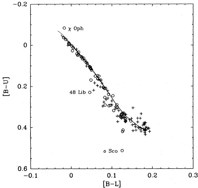
Fig. 6a. Reddening-free two-colour diagram of the stars in the Upper-Scorpius subgroup. Circles denote the established members of the association, plusses denote the remaining programme stars. The dashed line shows the ZAMS, whereas the full line gives the isochrone of age 5.5 million years
