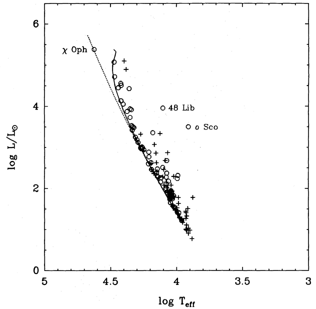
Fig. 6b. HR-diagram of the stars in the Upper-Scorpius subgroup. Circles denote the established members of the association, plusses denote the remaining programme stars. Note that the three member stars with strongly deviating position in the diagram are stars with a peculiar, emission-line spectrum ( \chi Oph and 48 Lib), and the bright giant o Sco (A 5 II)
