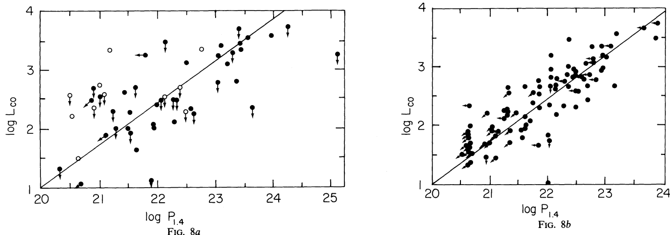
FIG. 8.—(a) Plot of the log of the CO luminosity (in \text{K km s}^{-1} \text{ kpc}^2 ) vs. the monochromatic radio power at 1.4 GHz ( \text{W Hz}^{-1} ) for the Seyfert galaxies in Table 2. We have used (whenever possible) 1.4 GHz continuum measurements made with low angular resolution to be certain that we have included all the radio flux from the galaxy. Such data are indicated by solid dots. Open dots are Seyfert galaxies for which only VLA A-configuration (high-resolution) data exist. In these cases, the 1.4 GHz data provide only a reliable measure of the radio power of the nucleus and may underestimate the total radio power of the galaxy (see notes to Table 2). The diagonal line is the estimated linear relation between \log L_{\text{CO}} and \log P_{1.4} for the non-Seyfert galaxies plotted in Fig. 7b. This linear regression was calculated using Schmitt's (1985) two-dimensional Kaplan-Meier estimator technique which properly treats upper limits in both variables. (b) As for (a) but for a sample of non-Seyfert galaxies. These galaxies were taken from the CO surveys of Stark et al. (1986) and Stark, Elmegreen, and Chance (1987) for normal galaxies, and from Sanders and Mirabel (1985), Sanders et al. (1986), and Young et al. (1984, 1986) for infrared-bright non-Seyferts. All the radio continuum data were low angular resolution and should represent the total radio power for each galaxy. The diagonal line is the Kaplan-Meier estimator of the linear regression between the two variables.
