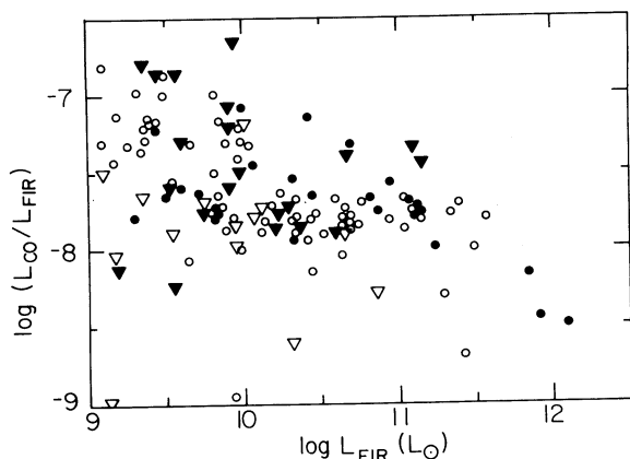
FIG. 6.—The log of the far-infrared luminosity (in L_\odot ) is plotted against the log of the ratio of the CO luminosity (in \text{K km s}^{-1} \text{ kpc}^2 ) and the far-infrared luminosity for Seyfert galaxies (solid points) and non-Seyfert galaxies (open points). CO detections are indicated by circles and nondetections (upper limits) by triangles. The Seyfert CO and IR data are taken from Tables 2 and 5. For the non-Seyferts, the CO data are from Stark et al. (1986), Sanders and Mirabel (1985), Sanders et al. (1986), and Young et al. (1984, 1986), and the IR data are from the IRAS Point Source Catalog. The Seyferts and non-Seyferts follow the same relationship between L_{\text{CO}} and L_{\text{FIR}} .
