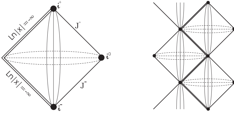
Figure 1.2: Left: the Penrose diagram for the metric given by (F-1). Right: the maximal analytic extension of the Penrose diagram.
