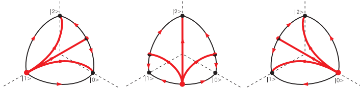
Figure 4.7: Part of the flow diagrams that are encountered as \chi moves from 0 to 2\pi in equations (4.18).
