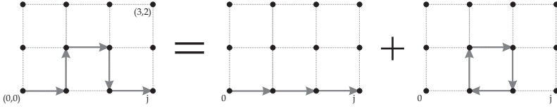
Figure 4.2: Different ways in which the points (0,0) and (3,0) can be connected. The summation over bond variables will in fact be independent of the path chosen, because the difference between two possible paths always consists of a summation around a closed loop. Such a closed-loop summation is sure to give a zero result in the absence of a magnetic field.
