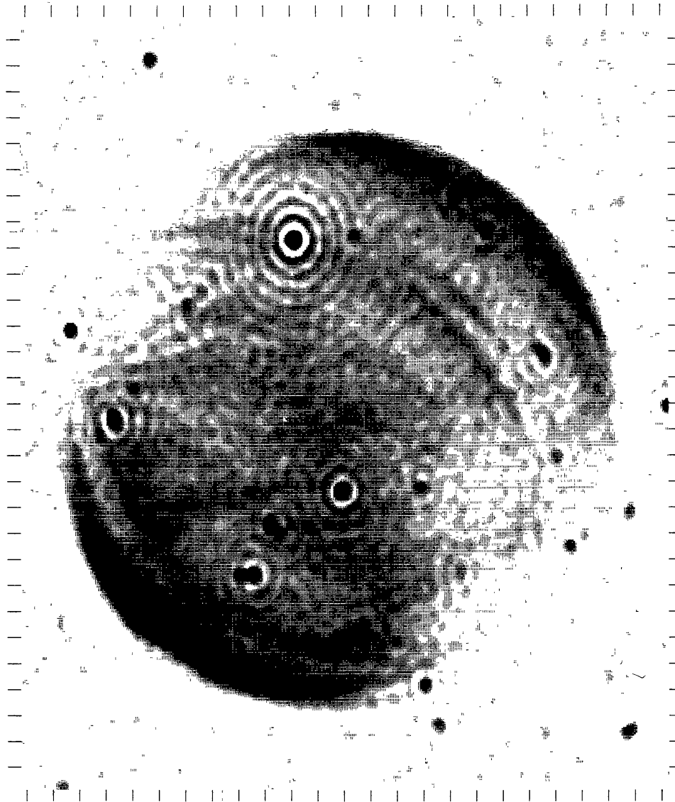
Figure 2. The 49 cm map of DA530.
