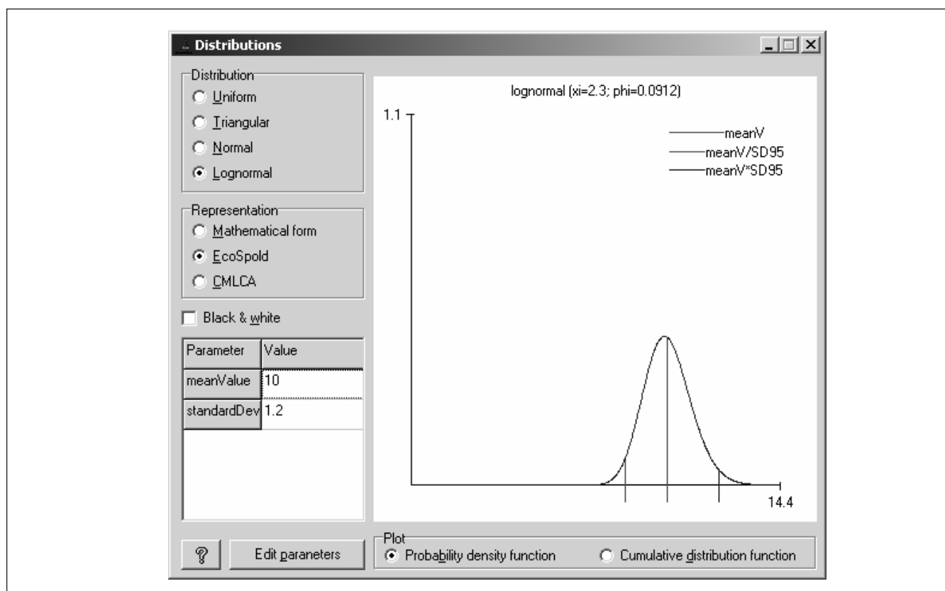
Fig. 5: Screen shot of the software-tool 'Distributions' for the lognormal distribution using the EcoSpold representation with the parameters meanValue = 10 and standardDeviation95 = 1.2
