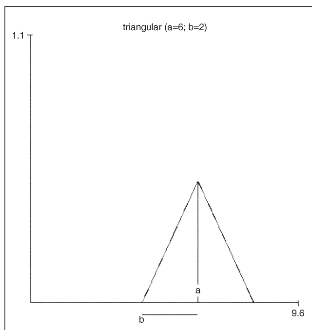
Fig. 2: The probability density function of the triangular distribution with parameters a=6 and b=2
