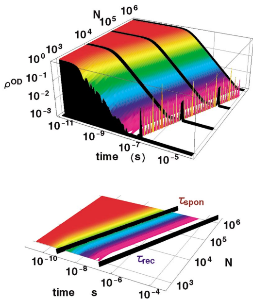
FIG. 3 (color). The time dependence of the entanglement between states |0\rangle and |2\rangle , |\rho^{\text{OD}}| , for different numbers of spins N at T = 10 K and t_{\text{rec}}/t_{\text{spon}} = 10^3 . In the bottom figure the decoherence time due to spontaneous symmetry breaking t_{\text{spon}} and the recurrence time t_{\text{rec}} are indicated.
