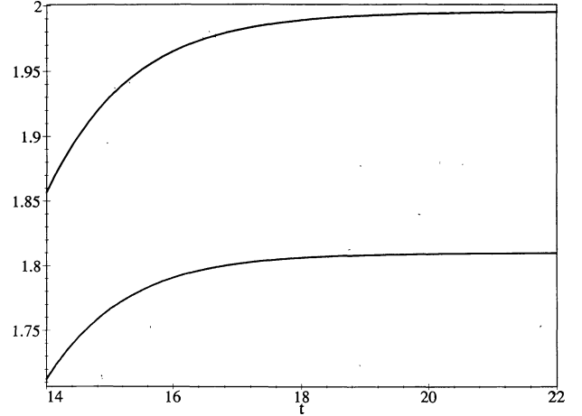
Fig. 1. Whitrow Randall relation as a function of time in the matter dominated era of Brans Dicke cosmology, shown for two different values of the coupling constant. The upper curve corresponds to w = 500 and the lower one to w = 10 . The axis t stands for the base logarithm of the cosmological time.
