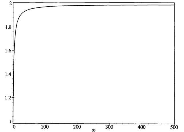
Fig. 2. Whitrow Randall relation value for today, as a function of the Brans Dicke coupling constant w .
