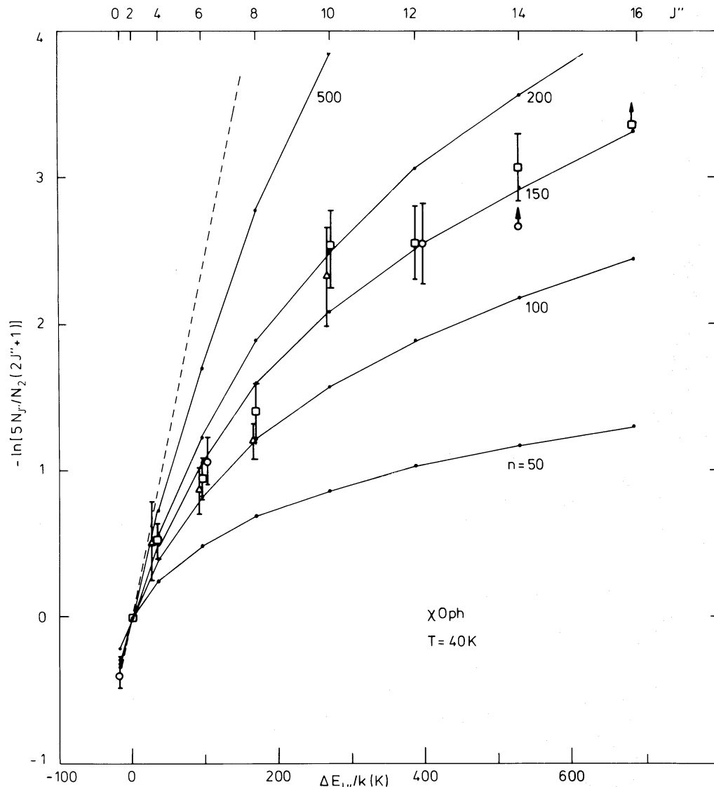
Figure 4. Observed relative rotational populations of C_2 with respect to that of the J'' = 2 level as functions of the excitation energy (or rotational quantum number J'' ) for the cloud in front of \chi Oph. For explanation of the symbols, see Fig. 3. The 1\sigma error bars are indicated. The theoretical populations (solid lines) at a kinetic temperature T = 40 K are shown for comparison at several densities n , assuming I = 1 and \sigma_0 = 2 \times 10^{-16} \text{ cm}^2 . The dashed line indicates the thermal distribution at 40 K. The best fit to the observational data is for n = 160 \text{ cm}^{-3} (or n\sigma_0/I = 3.2 \times 10^{-14} \text{ cm}^{-1} ).
