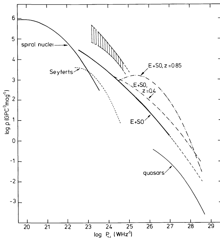
Figure 2. Schematic representation of the observed local RLF for: spiral galaxy nuclei (Hummel, 1980, thesis). Seyfert galaxies (Meurs, 1982, thesis), elliptical galaxies (Windhorst, 1983, thesis) and radio quasars (Fanti and Perola, 1977). Also shown are the elliptical RLF's at z \sim 0.4 and \sim 0.85 . The hatched area indicates the possible location of mJy objects responsible for the steepening of the count, for an assumed redshift of 0.4 \pm 0.2 .
