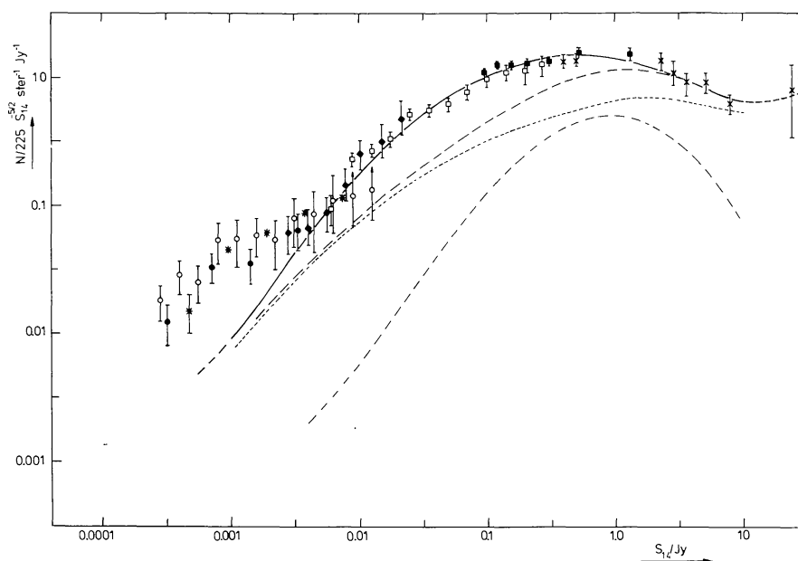
Figure 1. The 1.4 GHz differential source count normalized to a differential Euclidean count ( 225 S^{-5/2} \text{Sr}^{-1} \text{Jy}^{-1} ). References to older data ( S \gtrsim 10 mJy) can be found in Willis et al. (1977). Filled circles: Condon and Mitchell (1982), open circles: Windhorst et al. (1983 5\sigma sample, asterisks: Windhorst et al. 6.5\sigma sample, - . - : observed count of radio-loud quasars, ----: count of powerful radio ellipticals out to z \sim 0.85 , calculated from observed RLF, and assuming non-evolving RLF below \log P \sim 25.0 , -.-: sum of two above, —: total count of quasars and powerful ellipticals, with elliptical RLF extrapolated out to z \sim 1.5 (as described in text), and again assuming no evolution below \log P \sim 25.0 .
