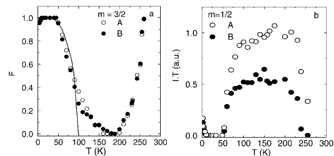
FIG. 3. (a) The T dependence of F for m = 3/2 . The maximal intensities for lines A and B are both normalized to one. Drawn line is a fit to the BCS gap function. (b) Intensities ( I ) times T for the decomposed m = 1/2 line, divided by the maximal value of IT of line A .
