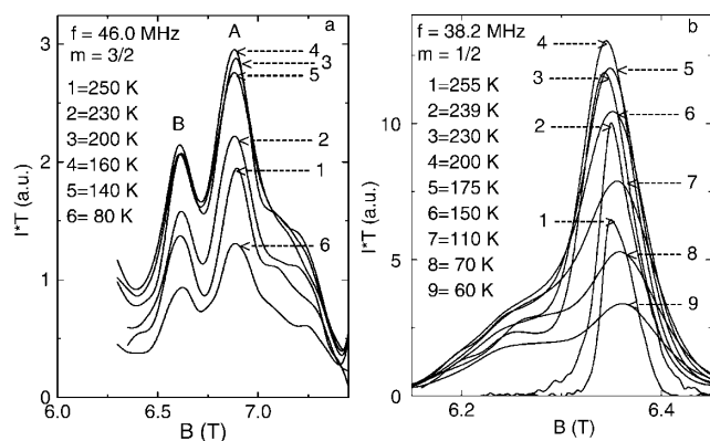
FIG. 1. ^{139}\text{La} NMR field profiles for (a) m = 3/2 (46.0 MHz) and (b) m = 1/2 (38.2 MHz) as a function of T . Arrows point to the line maxima. For m = 1/2 below 230 K a second line ( B ) comes up on the low field side of line A ; for m = 3/2 the two lines are visible from the start (below 250 K).
