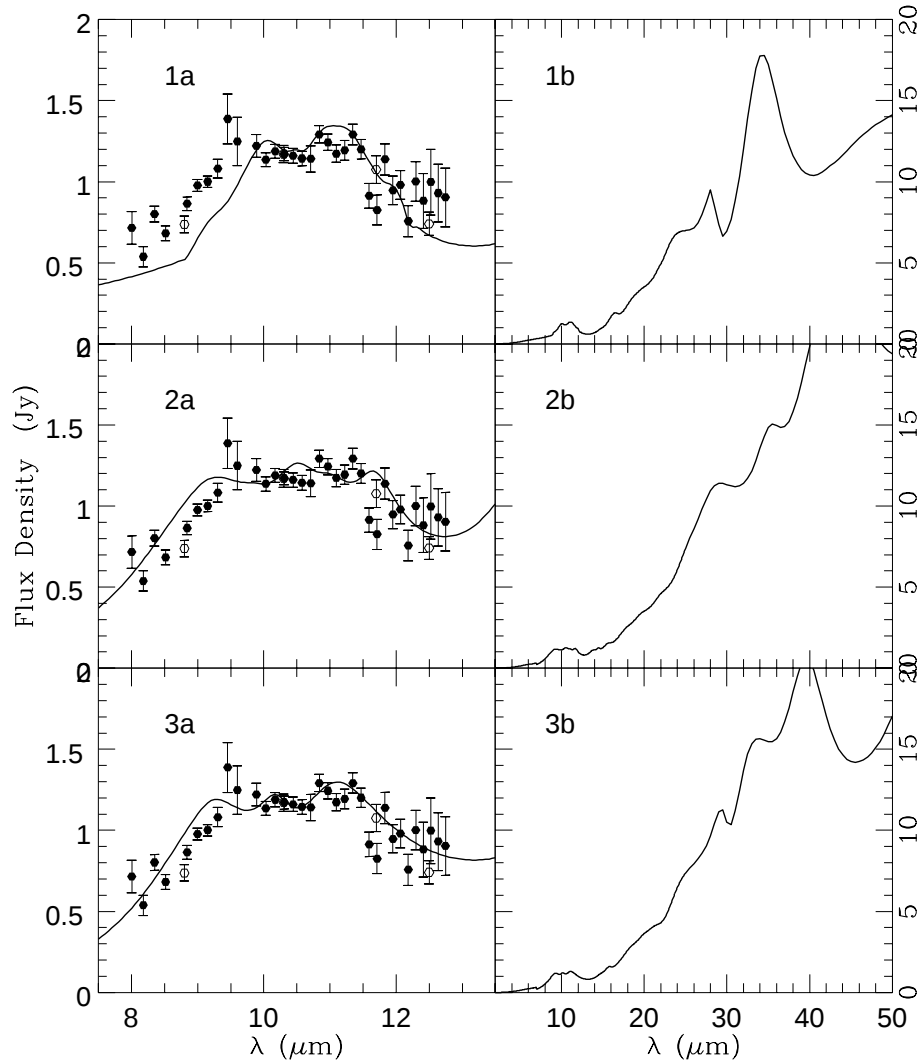
Fig. 12. The 10 \mu\text{m} silicate feature and the MIR emission band predicted from the crystalline silicate model in which the crystalline silicate mineral is: 1a, 1b crystalline olivine; 2a, 2b crystalline orthopyroxene; 3a, 3b crystalline clinopyroxene. All the other dust parameters are identical to those of Fig. 5.
