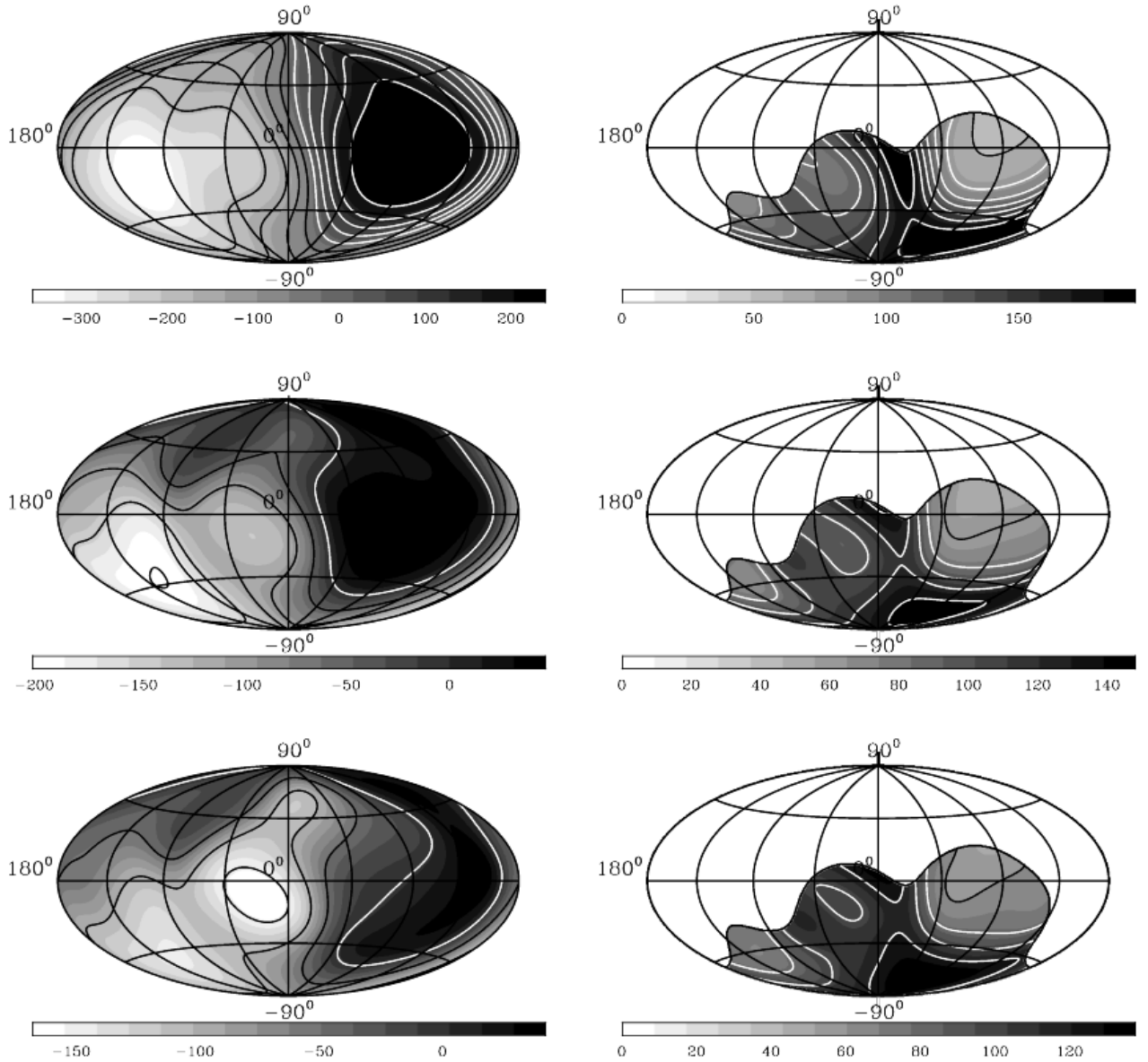
Fig. 8. Smoothed distributions of velocity and velocity dispersion of the CHVC ensemble. The panels on the left show the average velocity in the LSR (upper), GSR (middle), and LGSr (lower) reference frames, respectively. The panels on the right show the velocity dispersions, similarly arranged. Individual CHVCs in the ensemble were convolved with a Gaussian of true-angle dispersion of 20^\circ . White contours for the velocity and dispersion fields are drawn at values of 0, 50, ... \text{km s}^{-1} ; black ones are drawn at -50, -100, ... \text{km s}^{-1} . These smoothed representations of the observed situation can be compared with similarly sampled and smoothed representations of simulations, as described in the text.
