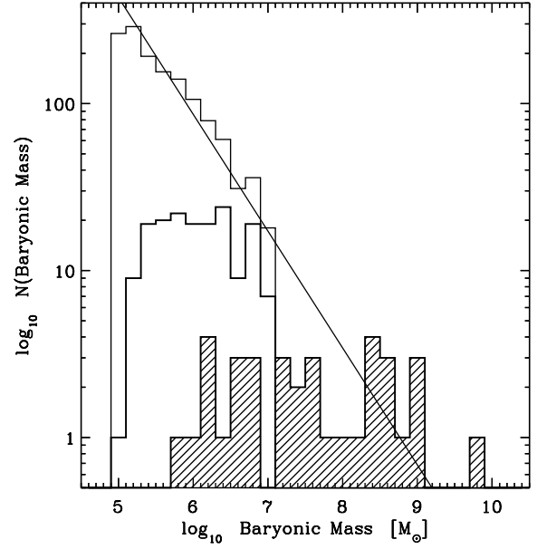
Fig. 28. Comparison of a model Local Group CHVC population with the population of Local Group galaxies. The distribution of H I masses of one of our best-fitting Local Group models, model #9 of Table 4, is plotted as a thin-line histogram after accounting for ram-pressure and tidal stripping and as a thick line after also accounting for Galactic obscuration and the finite sensitivities of the LDS and HIPASS observations. The Local Group galaxies (excluding M31 and the Galaxy) tabulated by Mateo (1998) are plotted as the hatched histogram after summing the H I mass with the stellar mass assuming M/L_B = 3 M_\odot/L_\odot . The diagonal line has the slope of the H I power-law mass function, \beta = -1.7 .
