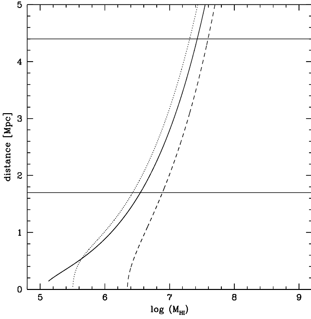
Fig. 13. Distances out to which simulated CHVCs would be detected in the HIPASS survey. The relation between the H I masses and maximum observable distance depends on the dark-matter fraction via the slope of the H I mass distribution of the CHVC population. The three curves refer to clouds with a mass-distribution slope of -2.0 , -1.6 , and -1.2 , as dotted, solid, and dashed lines, respectively. The \beta = -1.2 clouds are so diffuse that they fall below the HIPASS detection threshold for \log(M_{\text{HI}}) \lesssim 6.4 . The horizontal lines bracket distances to individual Sculptor Group galaxies.
