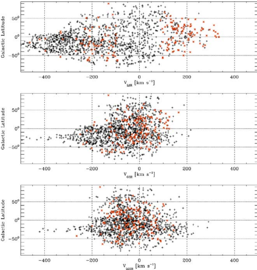
Fig. 22. Velocities plotted against galactic latitude for the ensemble of synthetic clouds corresponding to model #9 of a CHVC population in the Local Group. The kinematic distributions are indicated for three different kinematic reference frames, namely the LSR (upper), the GSR (middle), and the LGSR (lower panel). As in the simulated ( l, V ) distribution of Fig. 21, red symbols indicate unobscured clouds which are sufficiently bright to be detected by the Leiden/Dwingeloo or Parkes surveys, depending on the object declination, while black symbols refer to simulated clouds which are either too faint to be detected or obscured. The simulated ( b, V ) plot may be compared with the observed situation plotted in Fig. 7. (This figure is available in color in electronic form.)
