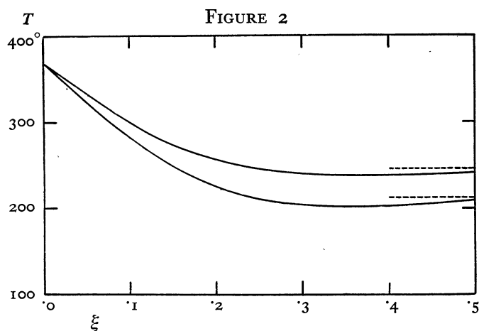
Temperature distributions as a function of \xi below the subsolar point.
