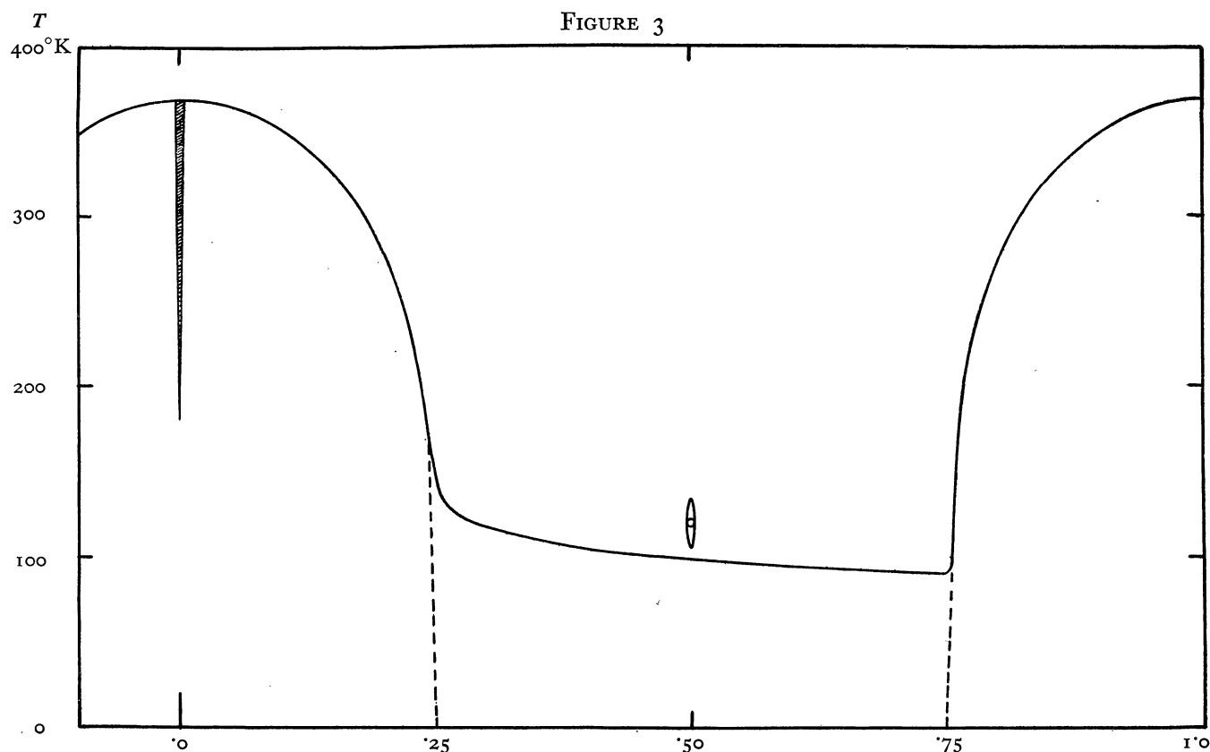
The calculated surface temperature of an area of the moon near the centre of the disc is shown during 11.1 lunation by the full-drawn curve. The dotted lines show the variation in the hypothetical case of zero conduction. The open circle represents PETTIT and NICHOLSON's observation during the lunar night. At full moon on left the variation during the 1939 eclipse is drawn on the same scale.
