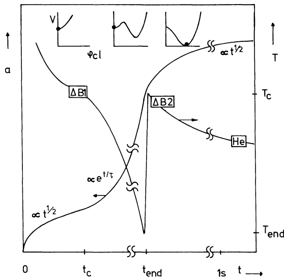
Fig. 1. Sketch of the history of the Universe during a first order phase transition: a is the scalefactor and T the equilibrium temperature (for adiabatic expansion T \propto a^{-1} ). Included representative forms of the effective potential V , whose minima are possible vacuum state (see text). Twice baryon number ( B ) non-conserving reactions could have generated a baryon-anti baryon asymmetry, but in the symmetric vacuum state there will be no net B generation during the \Delta B1 period. The observed B should thus be created after the reheating ( T_R \sim T_c ), which must be smooth in order to preserve a homogeneous Helium synthesis (see text)
