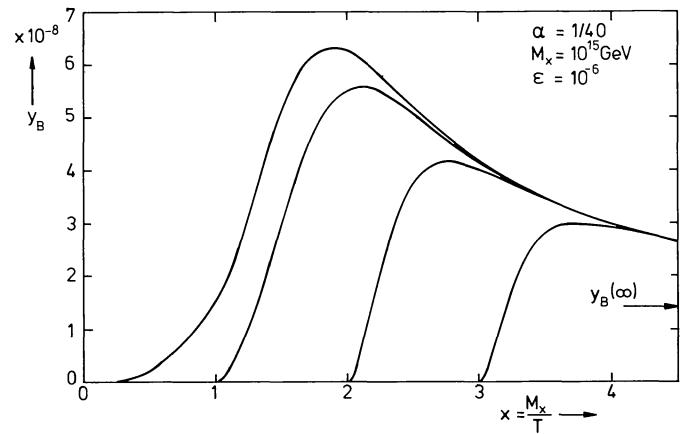
Fig. 2. The generation of the baryon number to photon ratio Y_B(x; x_0) , where x = M_X/T and M_X the mass of the B -violating boson, is calculated for a simple model, with CP violation parameter \epsilon . Earlier calculations (Kolb and Wolfram, 1980b) use symmetric starting conditions at x_0 = 0 . Finite temperature effects lead to phase transitions (PT), which give the boson a mass M_X only for T \leq T_c \sim M_X/g . The Y_B(x; x_0) evolution is calculated for realistic starting values after a second order PT ( x_0 \sim g \sim \frac{1}{2} ) or after the smooth reheating ending the period of supercooling of a first order PT ( x_0 \sim 1 ). The final Y_B values are given in Fig. 3
